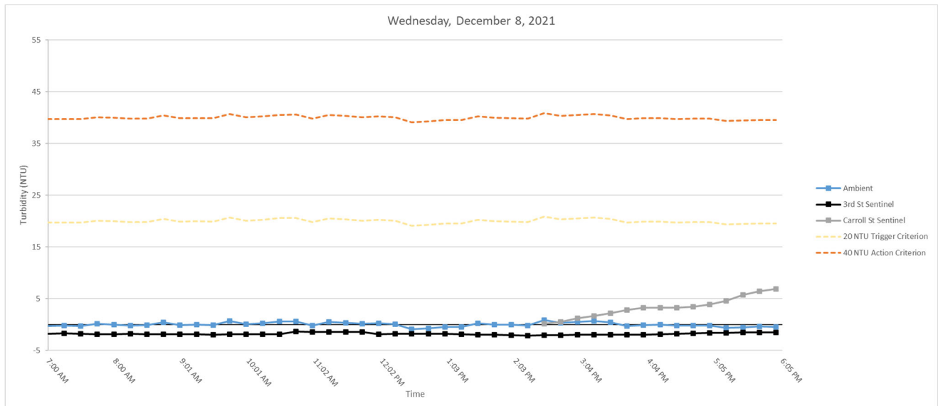
Figure 4. Hourly rolling average turbidity readings on Wednesday, December 8, 2021 from 7 AM to 6 PM.
