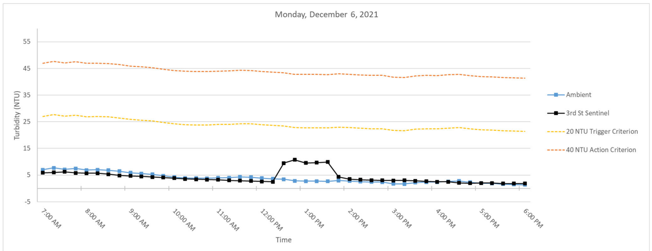
Figure 2. Hourly rolling average turbidity readings on Monday, December 6, 2021 from 7 AM to 6 PM.
