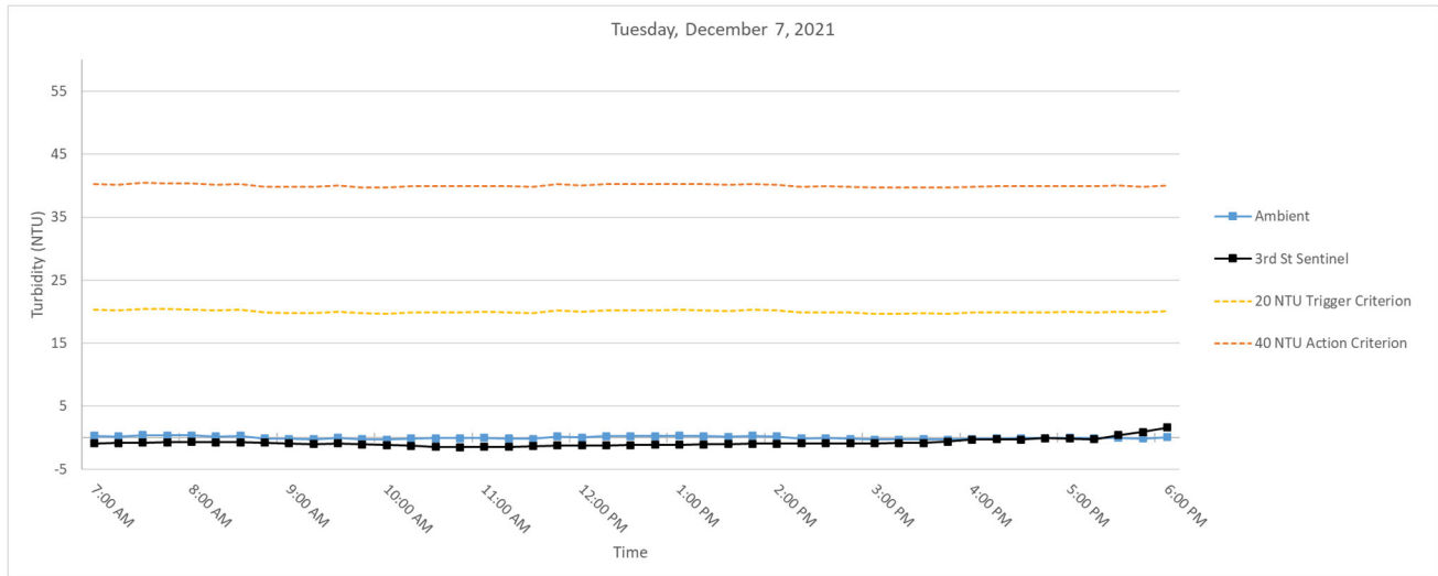
Figure 3. Hourly rolling average turbidity readings on Tuesday, December 7, 2021 from 7 AM to 6 PM.
