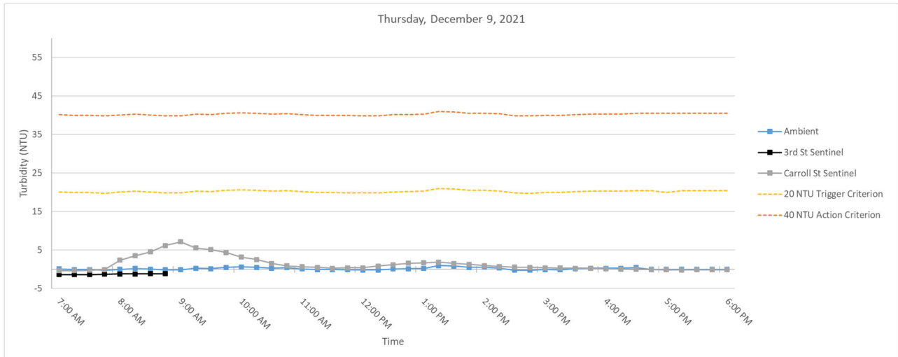
Figure 5. Hourly rolling average turbidity readings on Thursday, December 9, 2021 from 7 AM to 6 PM.
