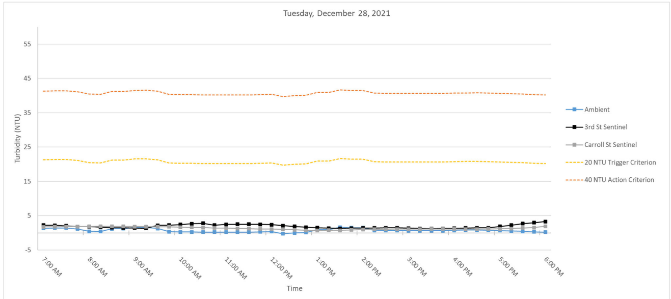
Figure 3. Hourly rolling average turbidity readings on Tuesday, December 28, 2021 from 7 AM to 6 PM.
