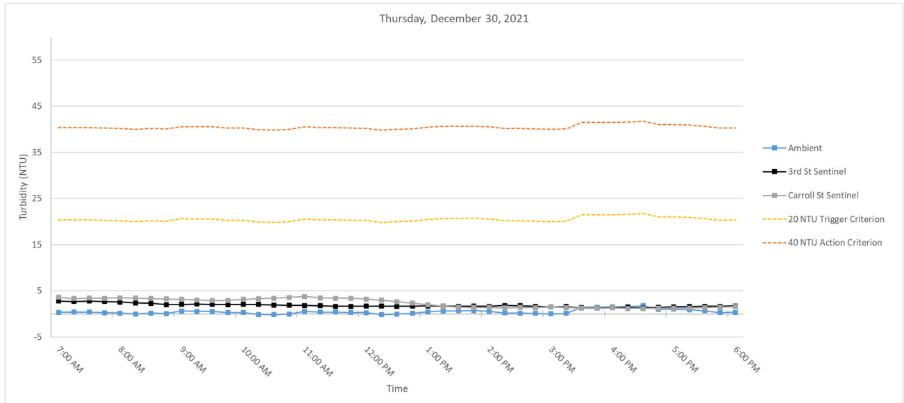
Figure 5. Hourly rolling average turbidity readings on Thursday, December 30, 2021 from 7 AM to 6 PM.
