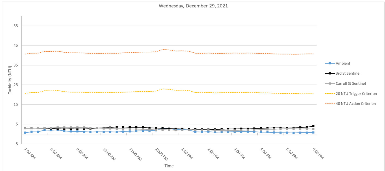
Figure 4. Hourly rolling average turbidity readings on Wednesday, December 29, 2021 from 7 AM to 6 PM.
