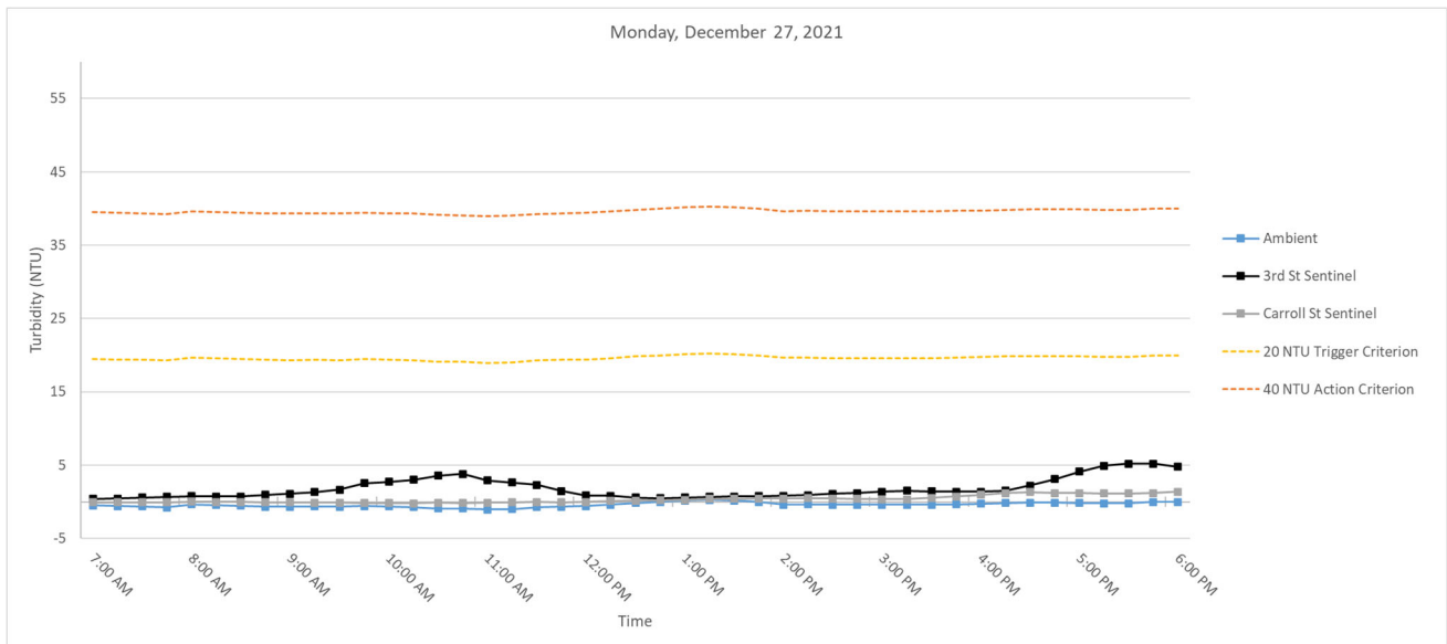
Figure 2. Hourly rolling average turbidity readings on Monday, December 27, 2021 from 7 AM to 6 PM.
