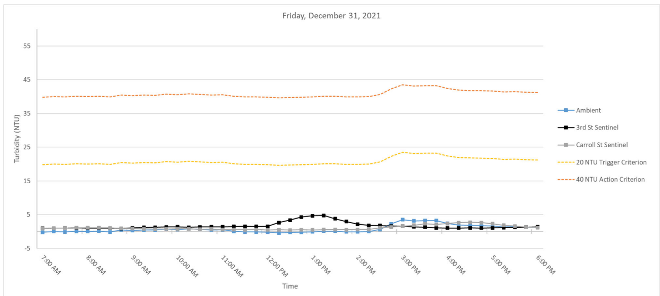
Figure 6. Hourly rolling average turbidity readings on Friday, December 31, 2021 from 7 AM to 6 PM.
