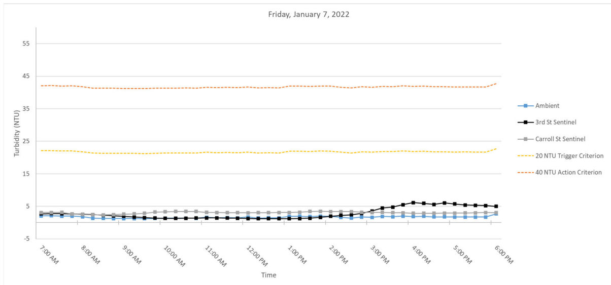
Figure 6. Hourly rolling average turbidity readings on Friday, January 7, 2022 from 7 AM to 6 PM.
