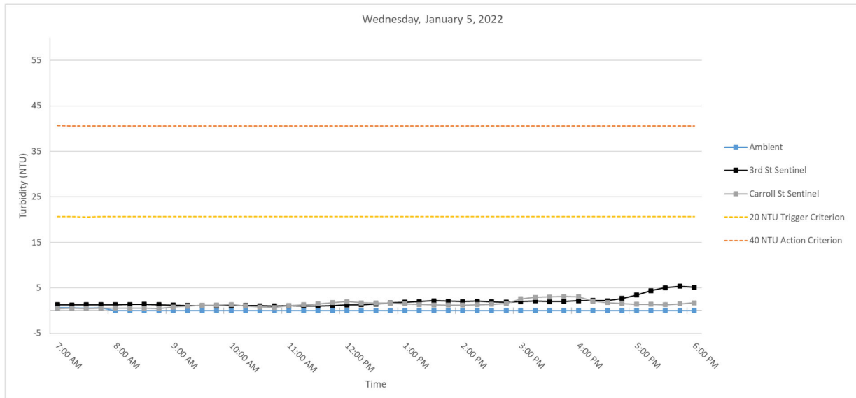
Figure 4. Hourly rolling average turbidity readings on Wednesday, January 5, 2022 from 7 AM to 6 PM.
