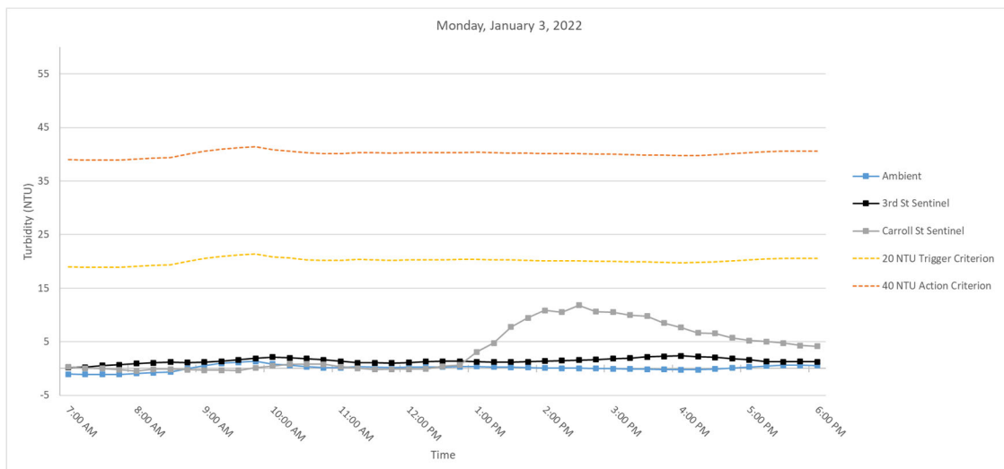
Figure 2. Hourly rolling average turbidity readings on Monday, January 3, 2022 from 7 AM to 6 PM.
