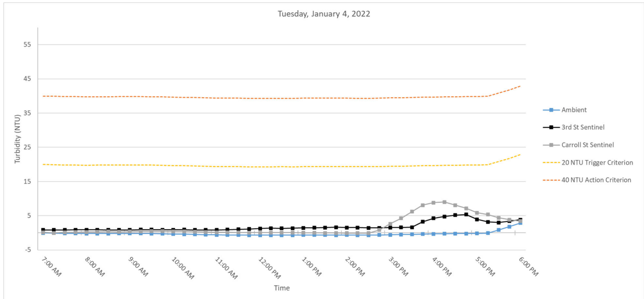
Figure 3. Hourly rolling average turbidity readings on Tuesday, January 4, 2022 from 7 AM to 6 PM.
