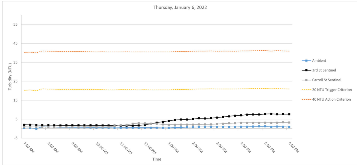
Figure 5. Hourly rolling average turbidity readings on Thursday, January 6, 2022 from 7 AM to 6 PM.
