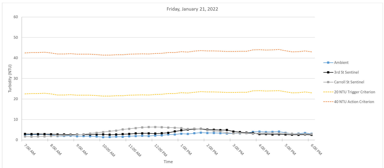
Figure 6. Hourly rolling average turbidity readings on Friday, January 21, 2022 from 7 AM to 6 PM.
