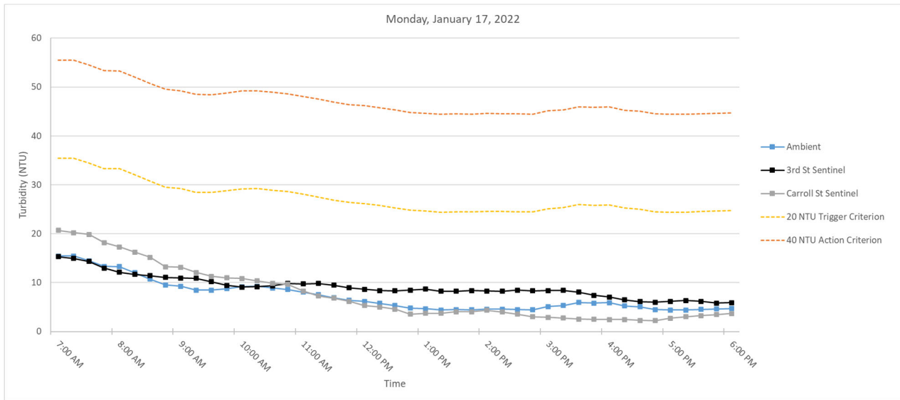
Figure 2. Hourly rolling average turbidity readings on Monday, January 17, 2022 from 7 AM to 6 PM.
