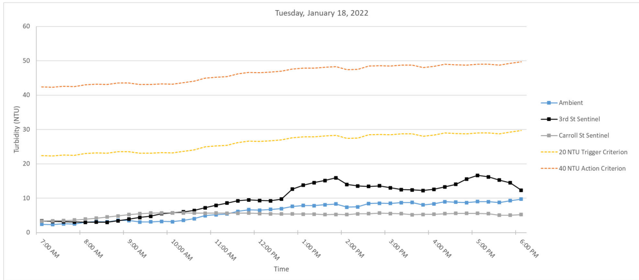
Figure 3. Hourly rolling average turbidity readings on Tuesday, January 18, 2022 from 7 AM to 6 PM.
