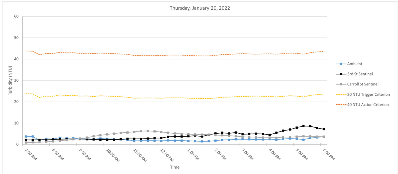
Figure 5. Hourly rolling average turbidity readings on Thursday, January 20, 2022 from 7 AM to 6 PM.
