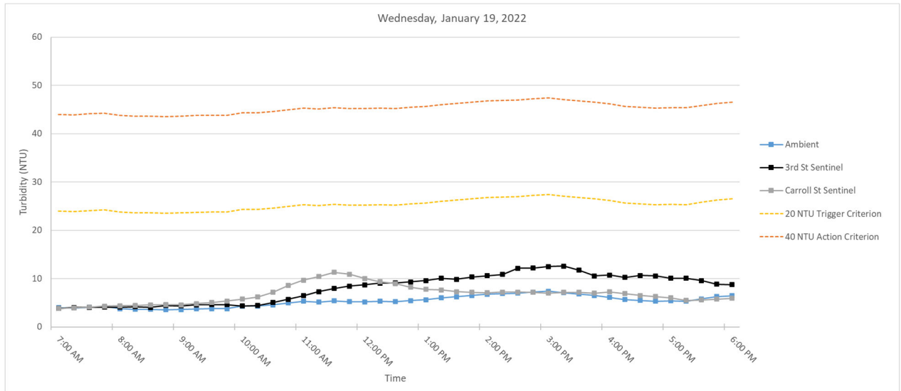
Figure 4. Hourly rolling average turbidity readings on Wednesday, January 19, 2022 from 7 AM to 6 PM.
