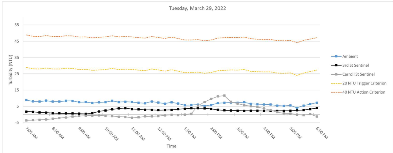
Figure 3. Hourly rolling average turbidity readings on Tuesday, March 29, 2022, from 7 AM to 6 PM.
