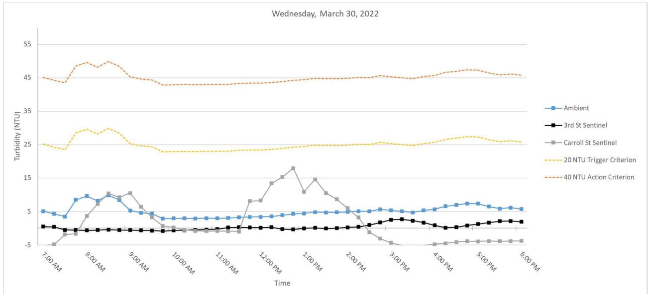
Figure 4. Hourly rolling average turbidity readings on Wednesday, March 30, 2022, from 7 AM to 6 PM.
