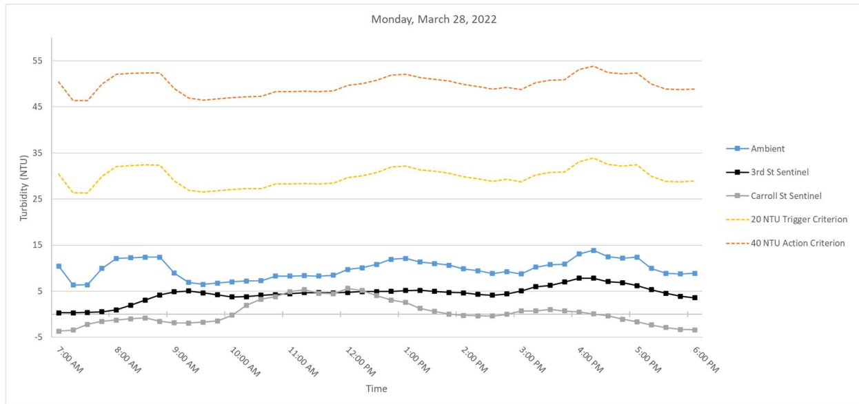
Figure 2. Hourly rolling average turbidity readings on Monday, March 28, 2022, from 7 AM to 6 PM.
