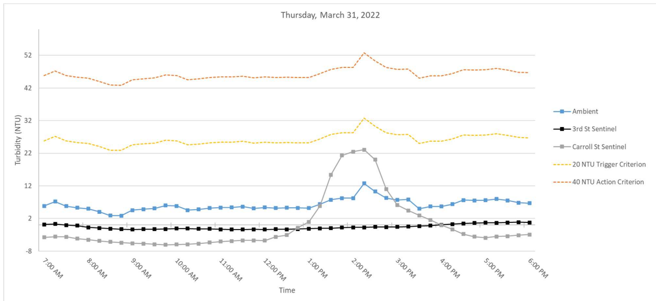
Figure 5. Hourly rolling average turbidity readings on Thursday, March 31, 2022, from 7 AM to 6 PM.
