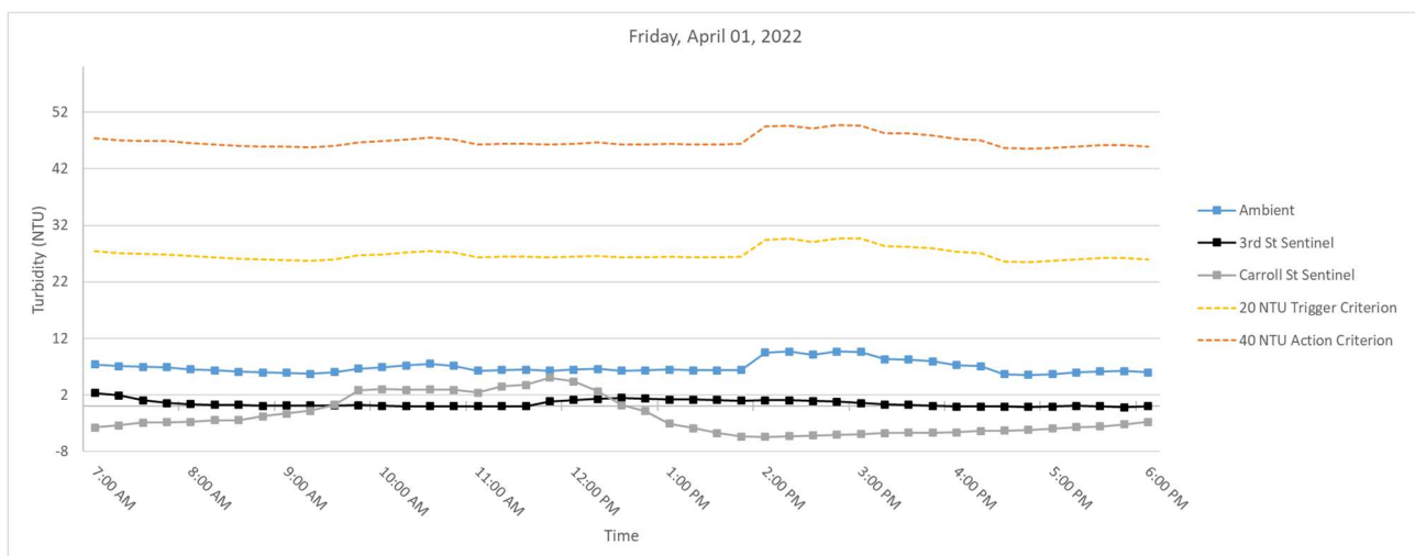
Figure 6. Hourly rolling average turbidity readings on Friday, April 01, 2022, from 7 AM to 6 PM.
