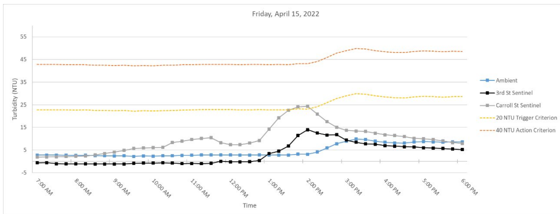
Figure 6. Hourly rolling average turbidity readings on Friday, April 15, 2022, from 7 AM to 6 PM.
