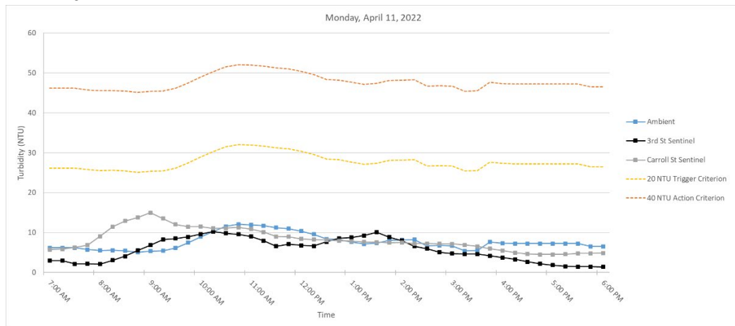
Figure 2. Hourly rolling average turbidity readings on Monday, April 11, 2022, from 7 AM to 6 PM.
