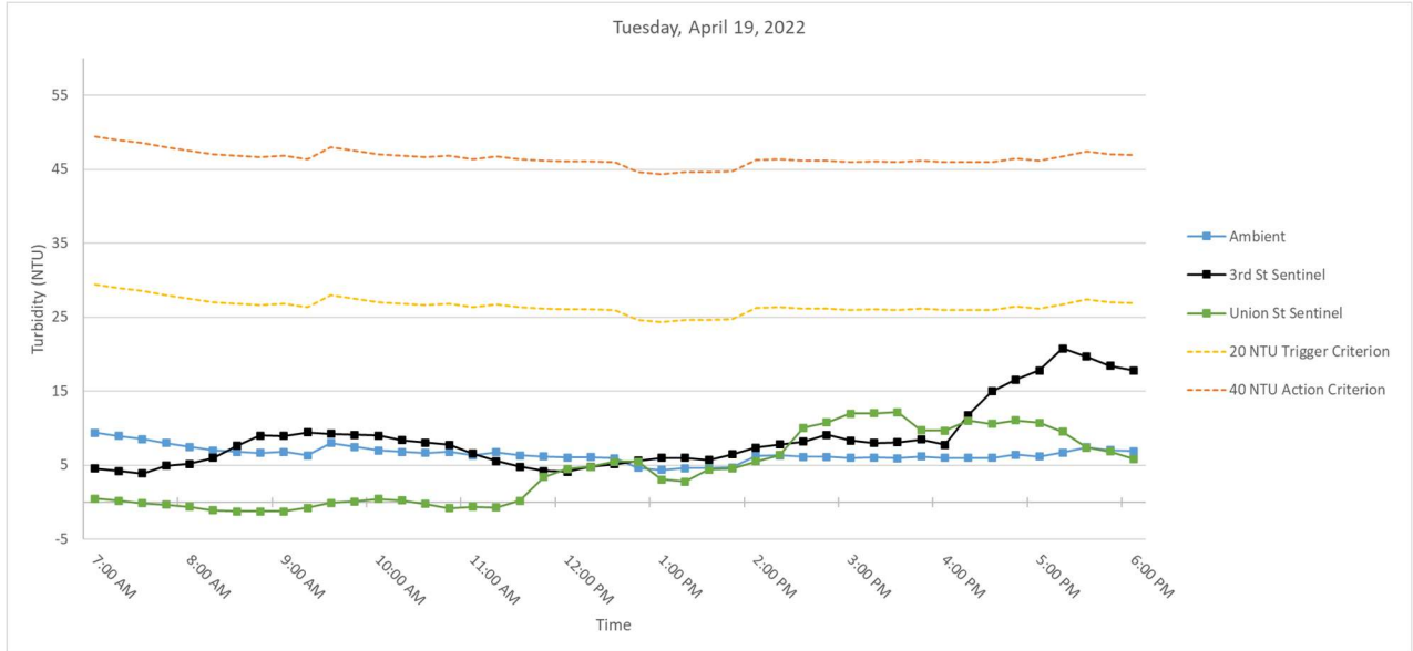
Figure 3. Hourly rolling average turbidity readings on Tuesday, April 19, 2022, from 7 AM to 6 PM.
