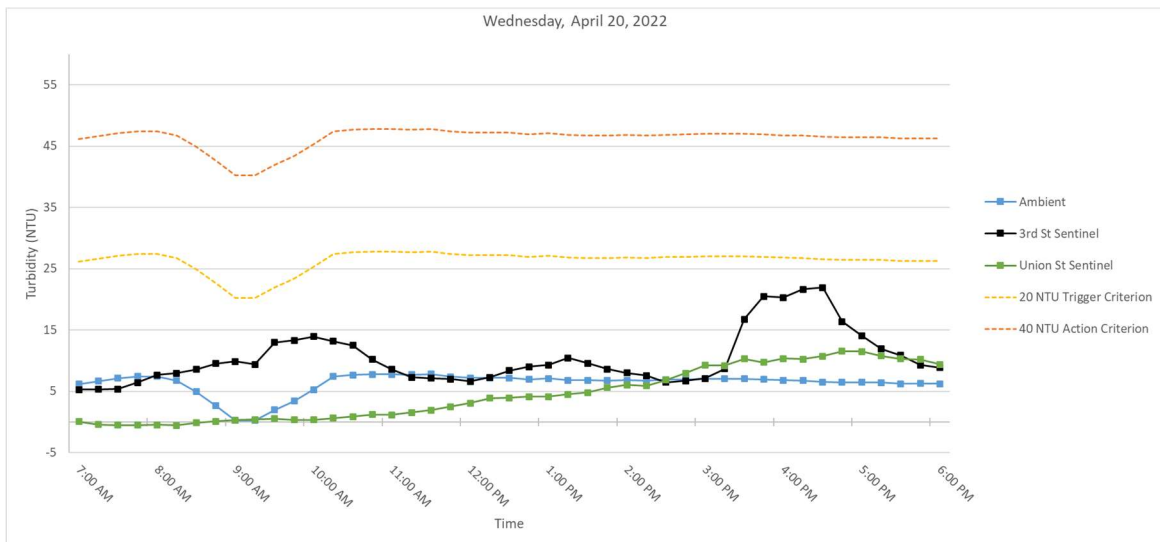
Figure 4. Hourly rolling average turbidity readings on Wednesday, April 20, 2022, from 7 AM to 6 PM.
