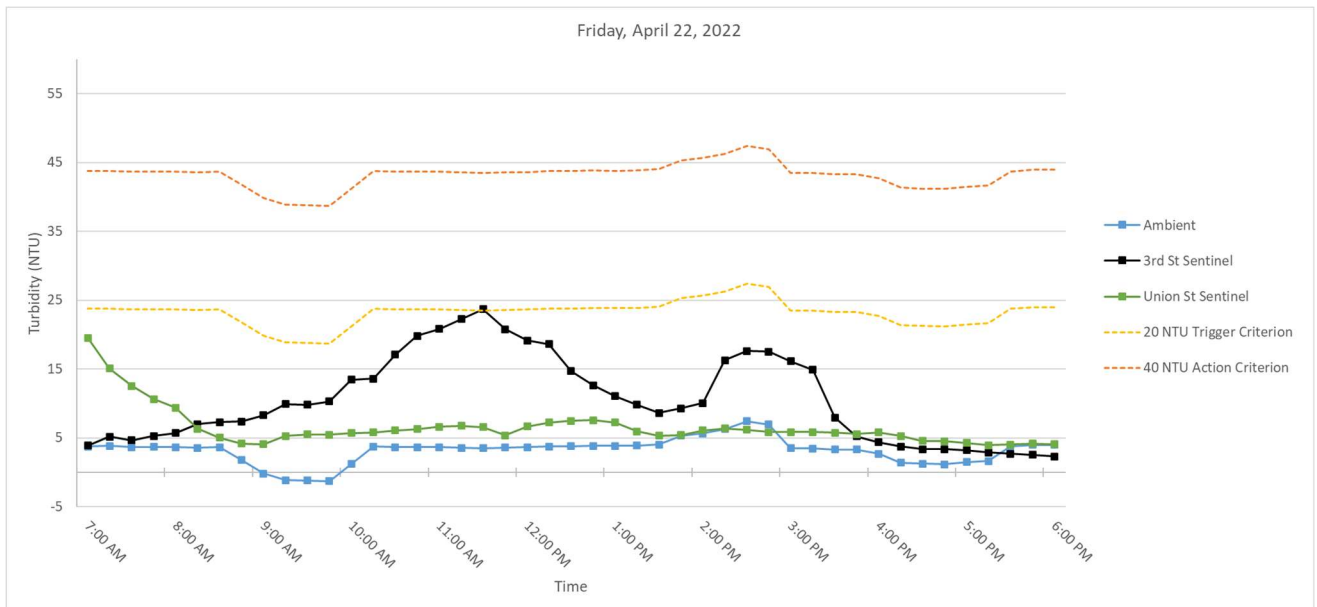
Figure 6. Hourly rolling average turbidity readings on Friday, April 22, 2022, from 7 AM to 6 PM.
