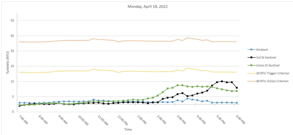
Figure 2. Hourly rolling average turbidity readings on Monday, April 18, 2022, from 7 AM to 6 PM.
