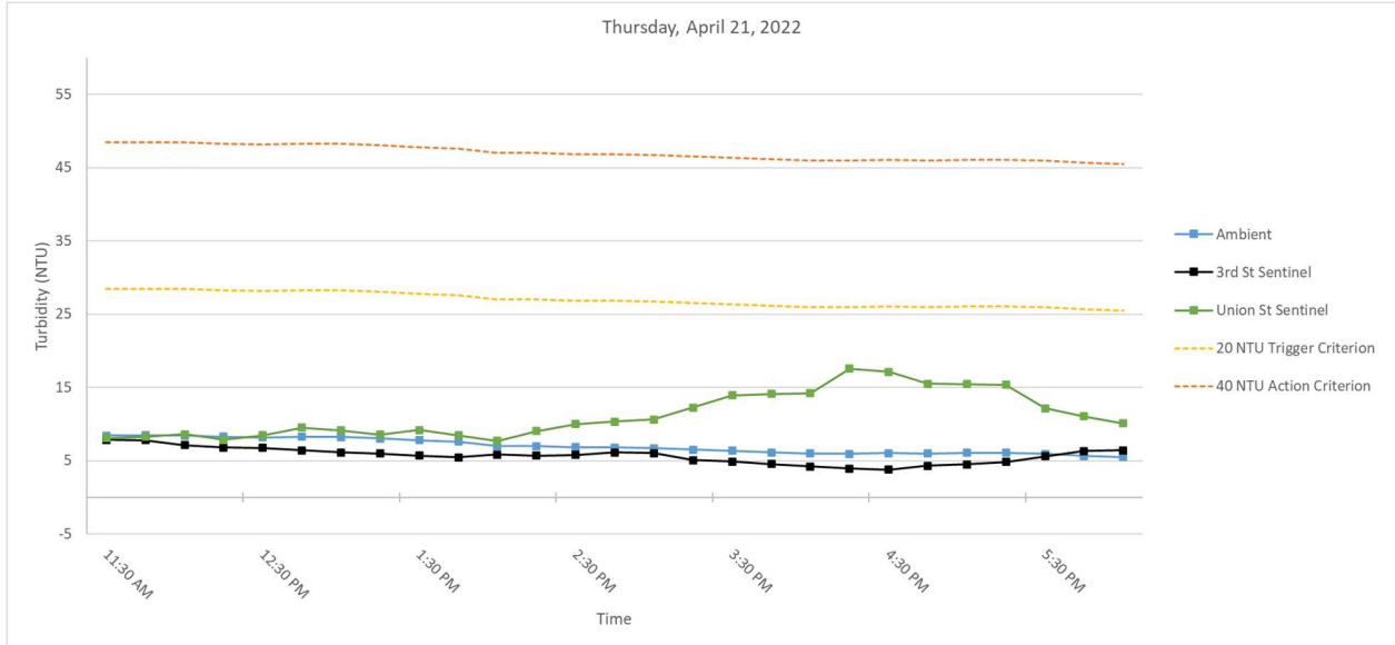
Figure 5. Hourly rolling average turbidity readings on Thursday, April 21, 2022, from 7 AM to 6 PM.
