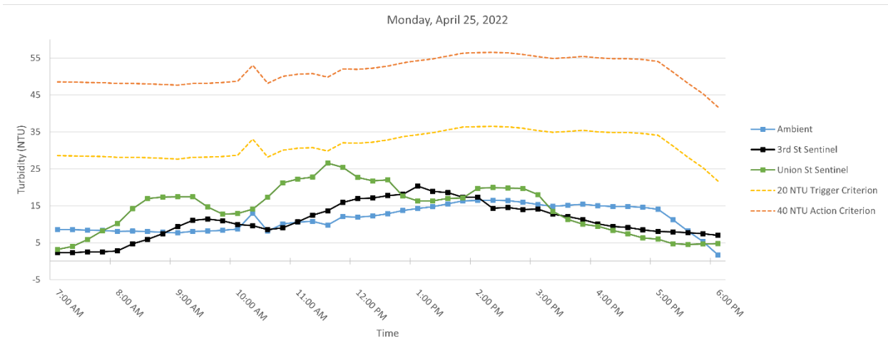
Figure 2. Hourly rolling average turbidity readings on Monday, April 25, 2022, from 7 AM to 6 PM.
