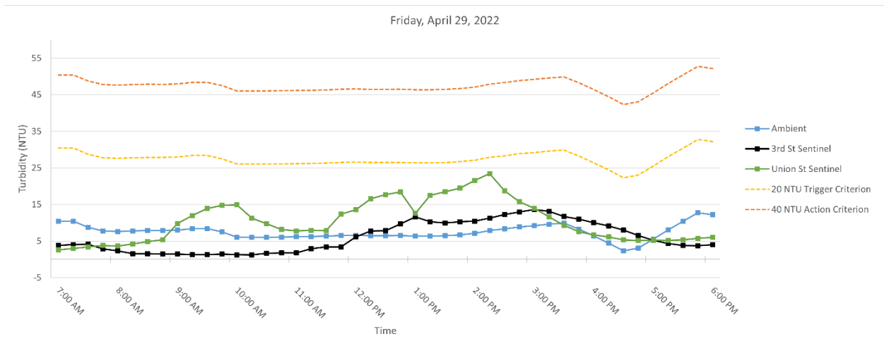
Figure 6. Hourly rolling average turbidity readings on Friday, April 29, 2022, from 7 AM to 6 PM.
