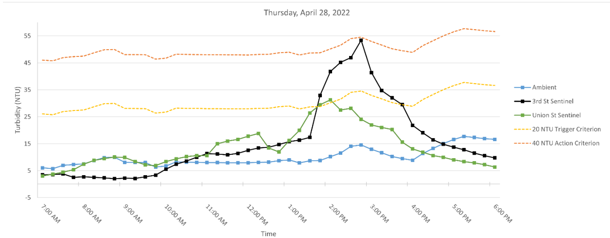
Figure 5. Hourly rolling average turbidity readings on Thursday, April 28, 2022, from 7 AM to 6 PM.
