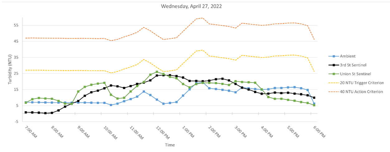
Figure 4. Hourly rolling average turbidity readings on Wednesday, April 27, 2022, from 7 AM to 6 PM.
