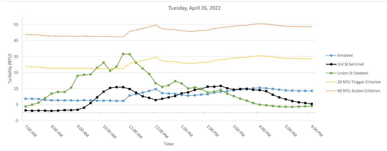
Figure 3. Hourly rolling average turbidity readings on Tuesday, April 26, 2022, from 7 AM to 6 PM.
