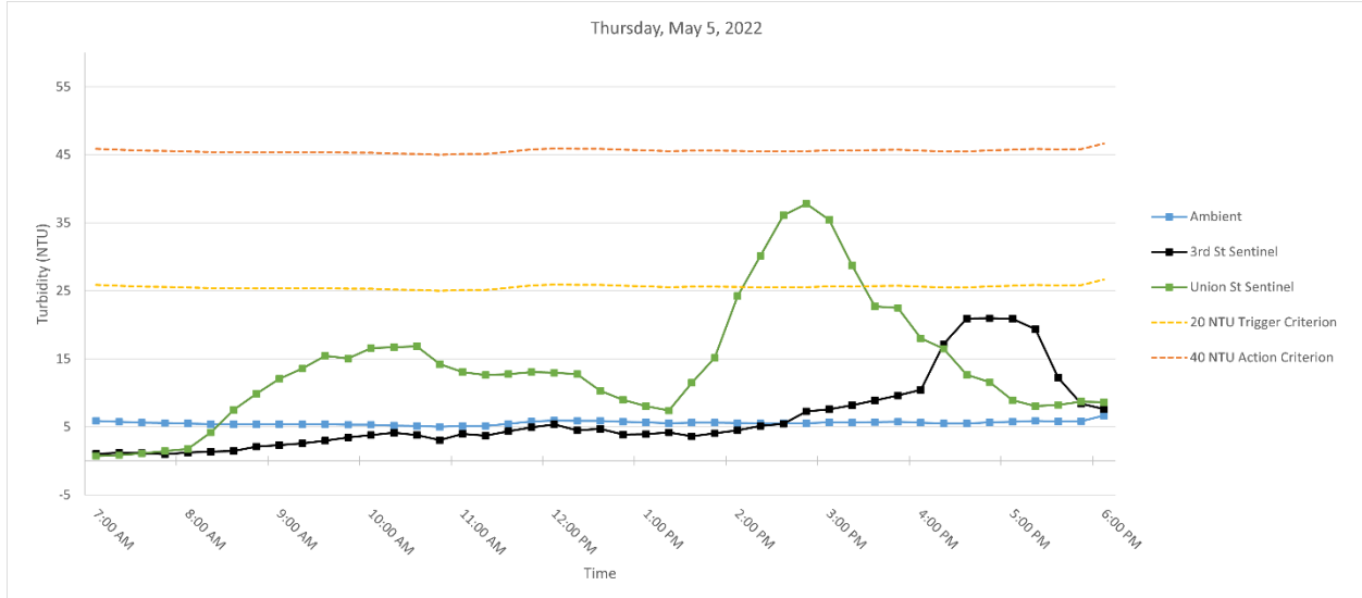
Figure 5. Hourly rolling average turbidity readings on Thursday, May 5, 2022, from 7 AM to 6 PM.
