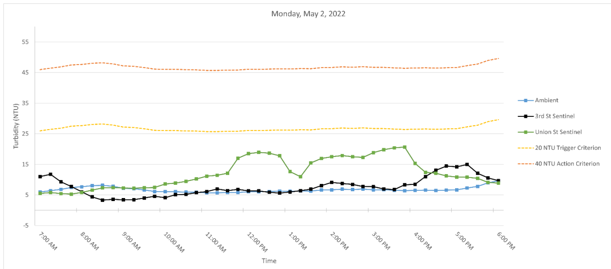
Figure 2. Hourly rolling average turbidity readings on Monday, May 2, 2022, from 7 AM to 6 PM.
