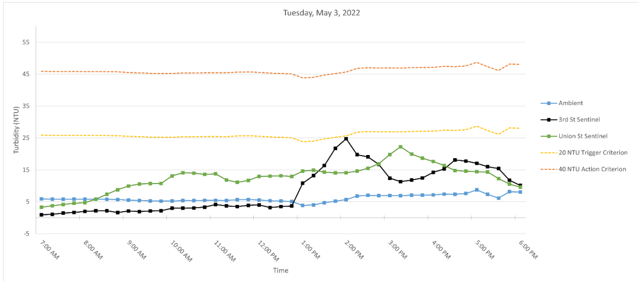
Figure 3. Hourly rolling average turbidity readings on Tuesday, May 3, 2022, from 7 AM to 6 PM.
