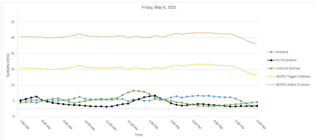
Figure 6. Hourly rolling average turbidity readings on Friday, May 6, 2022, from 7 AM to 6 PM.
