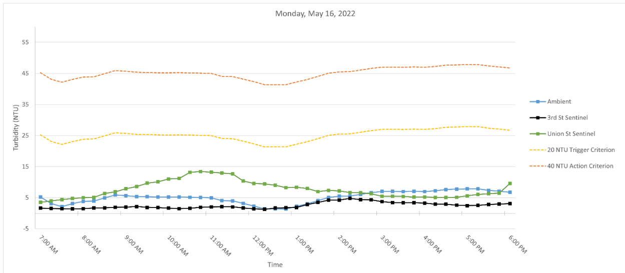
Figure 2. Hourly rolling average turbidity readings on Monday, May 16, 2022, from 7 AM to 6 PM.
