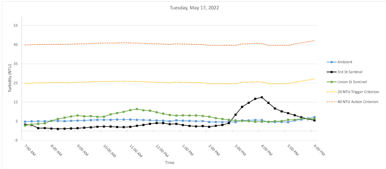
Figure 3. Hourly rolling average turbidity readings on Tuesday, May 17, 2022, from 7 AM to 6 PM.
