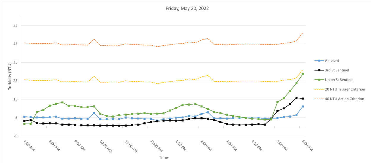
Figure 6. Hourly rolling average turbidity readings on Friday, May 20, 2022, from 7 AM to 6 PM.
