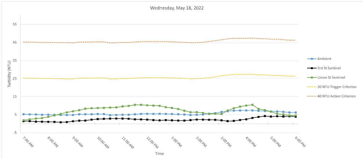
Figure 4. Hourly rolling average turbidity readings on Wednesday, May 18, 2022, from 7 AM to 6 PM.
