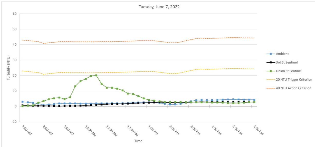
Figure 3. Hourly rolling average turbidity readings on Tuesday, June 7, 2022, from 7 AM to 6 PM.
