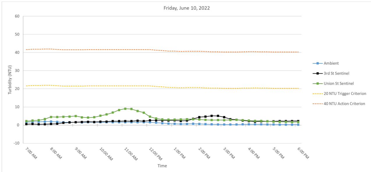
Figure 6. Hourly rolling average turbidity readings on Friday, June 10, 2022, from 7 AM to 6 PM.
