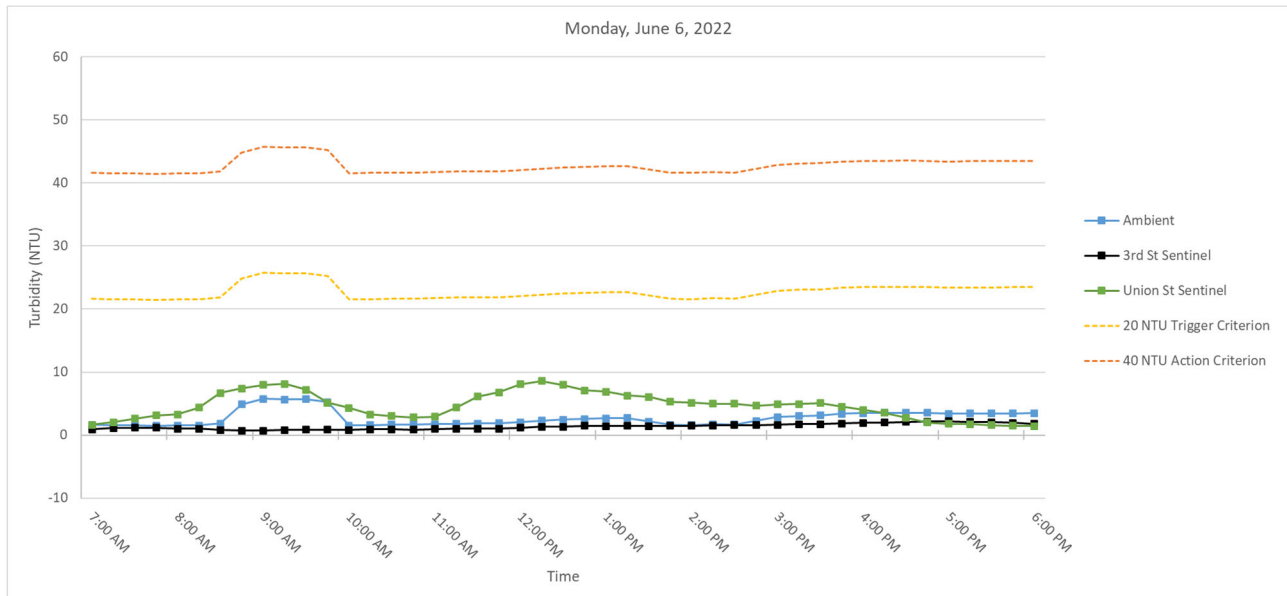
Figure 2. Hourly rolling average turbidity readings on Monday, June 6, 2022, from 7 AM to 6 PM.
