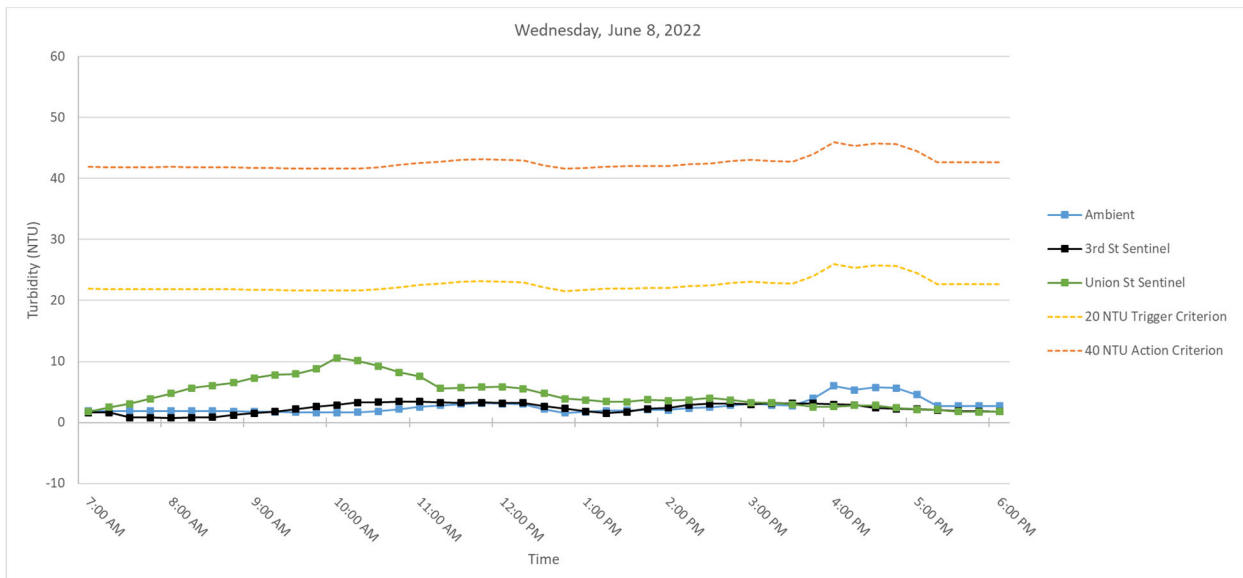
Figure 4. Hourly rolling average turbidity readings on Wednesday, June 8, 2022, from 7 AM to 6 PM.
