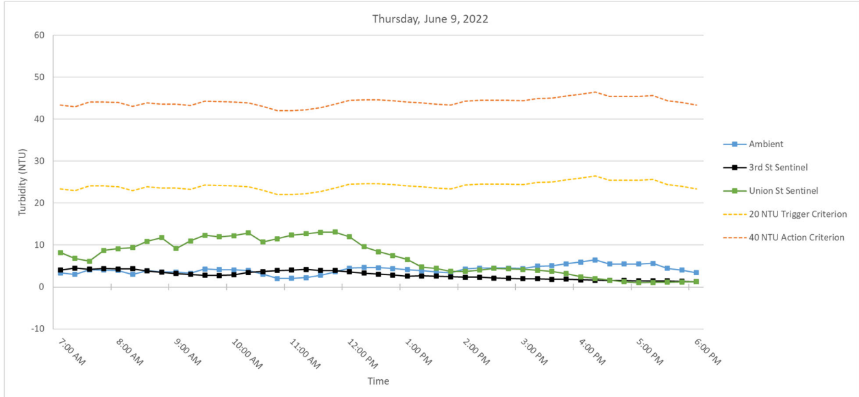
Figure 5. Hourly rolling average turbidity readings on Thursday, June 9, 2022, from 7 AM to 6 PM.
