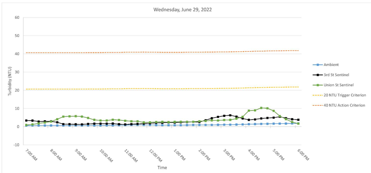
Figure 4. Hourly rolling average turbidity readings on Wednesday, June 29, 2022, from 7 AM to 6 PM.
