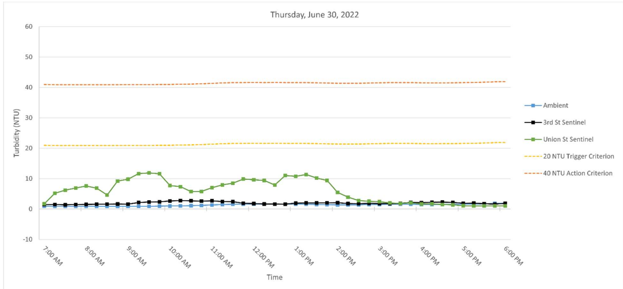
Figure 5. Hourly rolling average turbidity readings on Thursday, June 30, 2022, from 7 AM to 6 PM.
