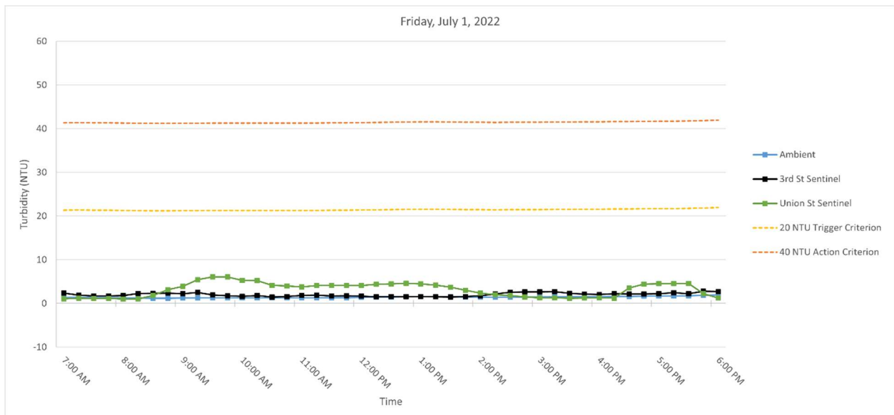
Figure 6. Hourly rolling average turbidity readings on Friday, July 1, 2022, from 7 AM to 6 PM.
