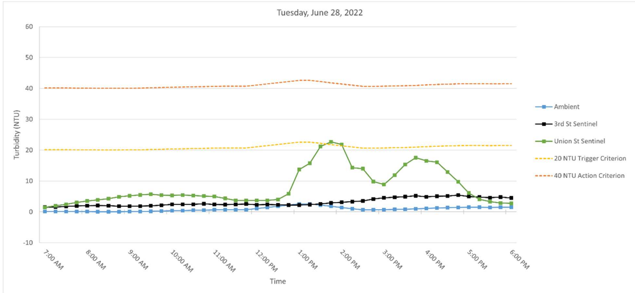
Figure 3. Hourly rolling average turbidity readings on Tuesday, June 28, 2022, from 7 AM to 6 PM.
