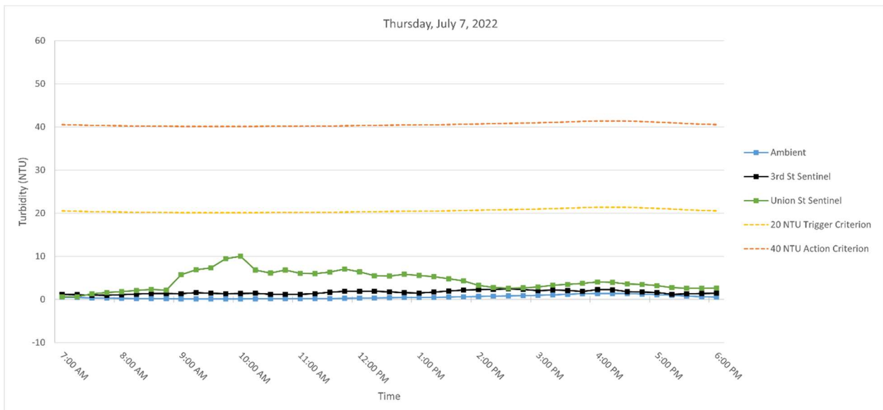
Figure 5. Hourly rolling average turbidity readings on Thursday, July 7, 2022, from 7 AM to 6 PM.
