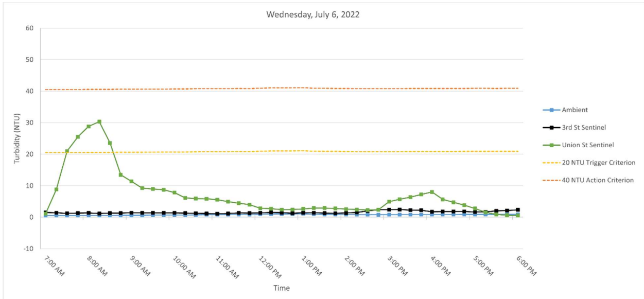
Figure 4. Hourly rolling average turbidity readings on Wednesday, July 6, 2022, from 7 AM to 6 PM.
