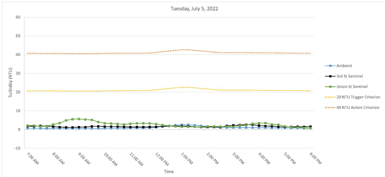
Figure 3. Hourly rolling average turbidity readings on Tuesday, July 5, 2022, from 7 AM to 6 PM.
