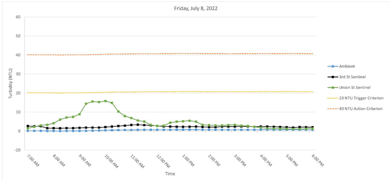
Figure 6. Hourly rolling average turbidity readings on Friday, July 8, 2022, from 7 AM to 6 PM.
