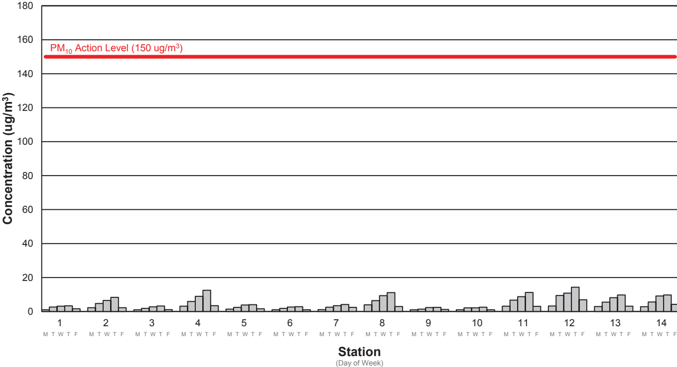
Average PM10 Concentration Week 152: 10/9/2023 - 10/13/2023
