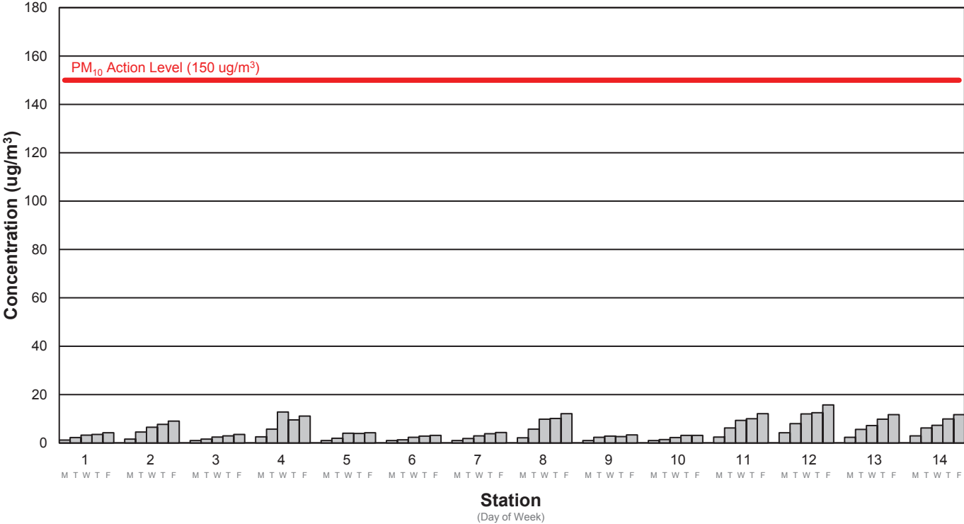
Average PM10 Concentration Week 154: 10/23/2023 - 10/27/2023
