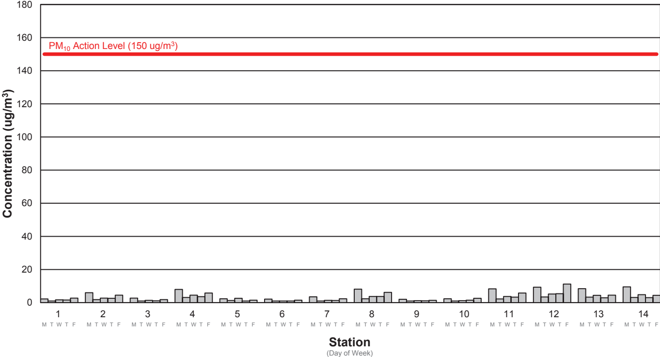
Average PM10 Concentration Week 155: 10/30/2023 - 11/3/2023
