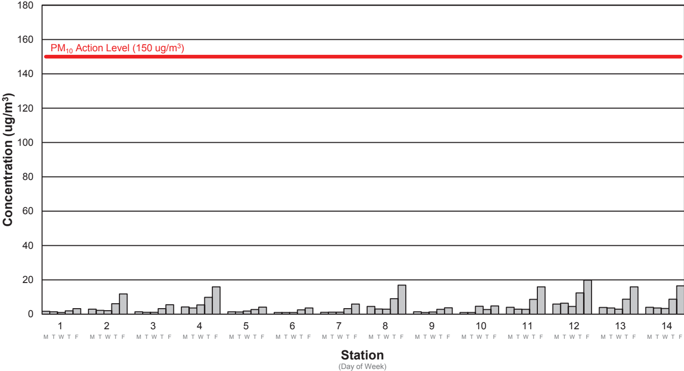
Average PM10 Concentration Week 160: 12/4/2023 - 12/8/2023
