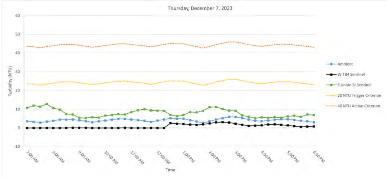
Figure 5. Hourly rolling average turbidity readings on Thursday, December 7, 2023, from 7 AM to 6 PM.
