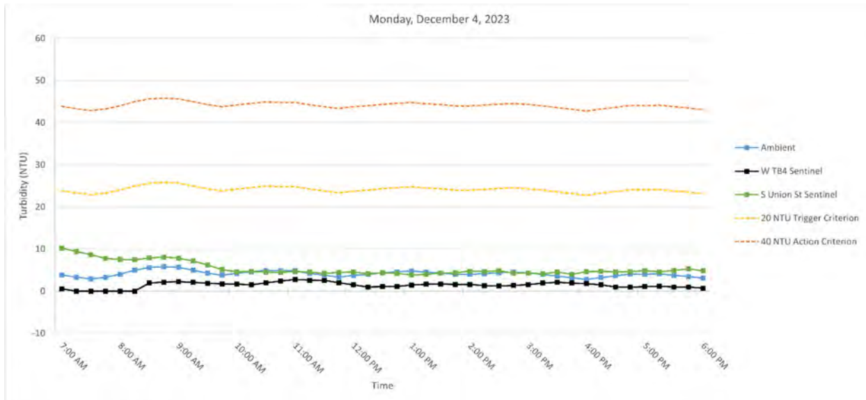
Figure 3. Hourly rolling average turbidity readings on Monday, December 4, 2023, from 7 AM to 6 PM.
