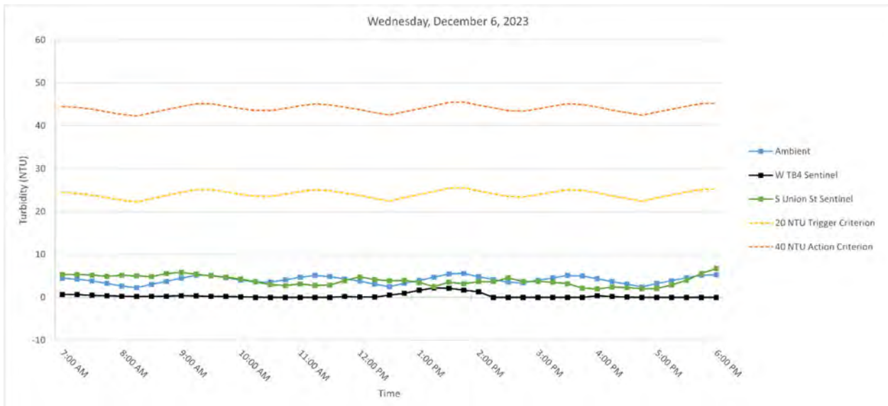
Figure 4. Hourly rolling average turbidity readings on Wednesday, December 6, 2023, from 7 AM to 6 PM.
