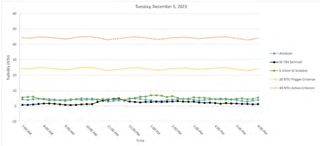
Figure 3. Hourly rolling average turbidity readings on Tuesday, December 5, 2023, from 7 AM to 6 PM.
