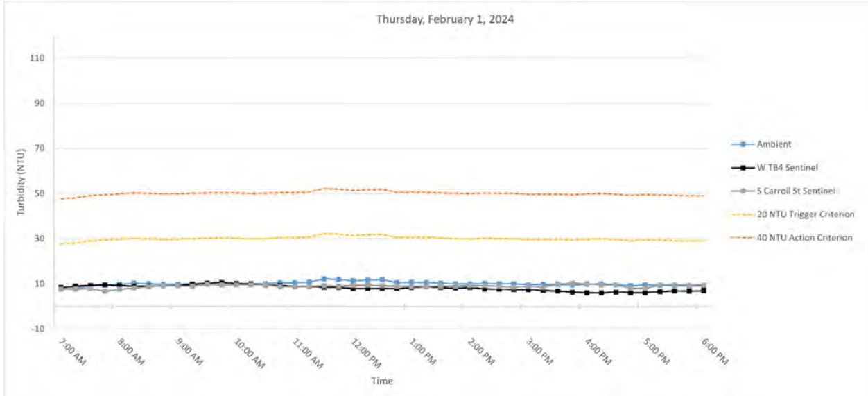
Figure 5. Hourly rolling average turbidity readings on Thursday, February 1, 2024, from 7 AM to 6 PM.
