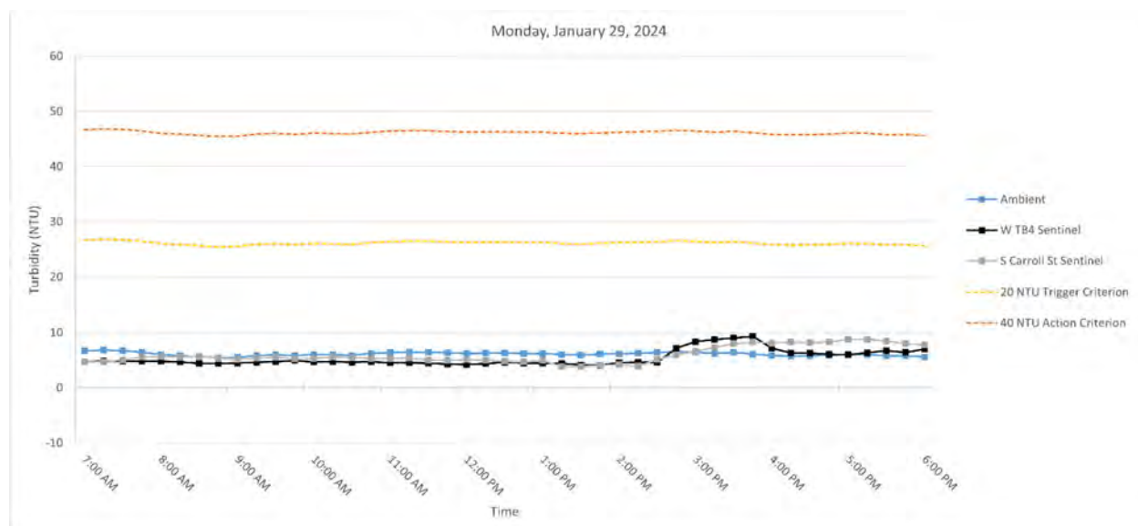
Figure 3. Hourly rolling average turbidity readings on Monday, January 29, 2024, from 7 AM to 6 PM.
