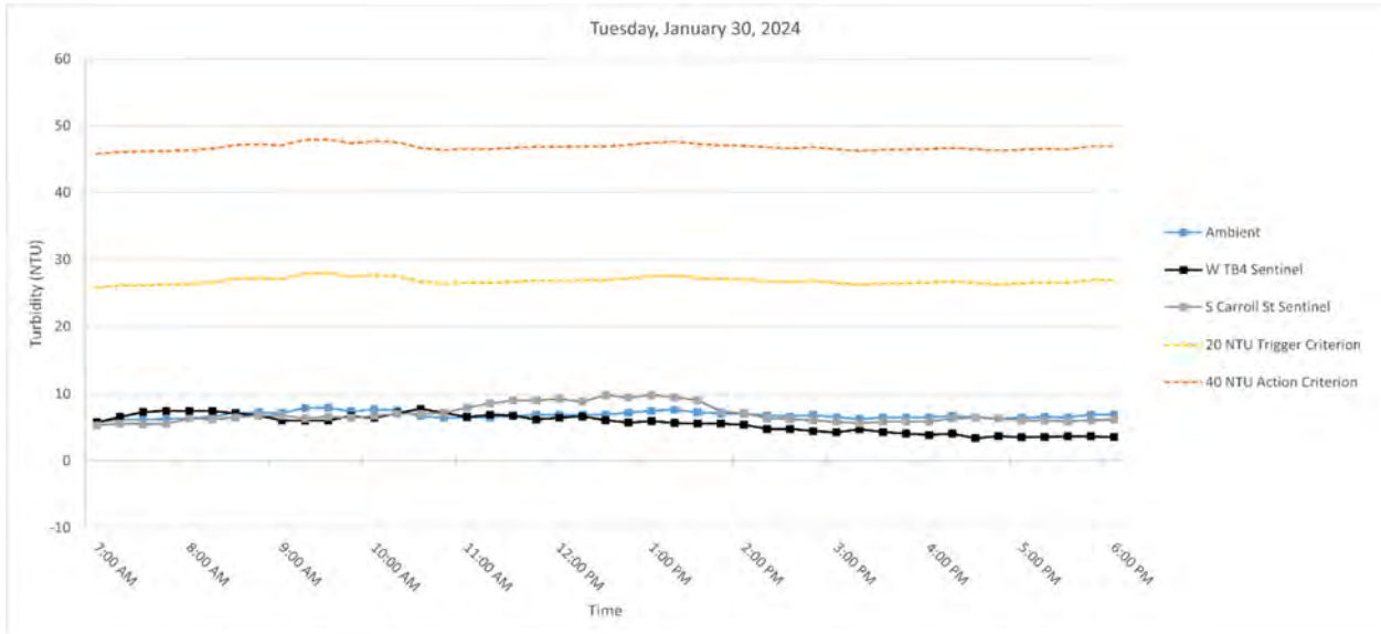
Figure 3. Hourly rolling average turbidity readings on Tuesday, January 30, 2024, from 7 AM to 6 PM.
