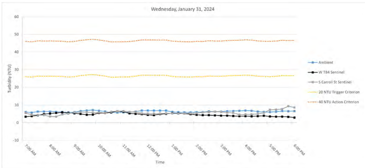
Figure 4. Hourly rolling average turbidity readings on Wednesday, January 31, 2024, from 7 AM to 6 PM.
