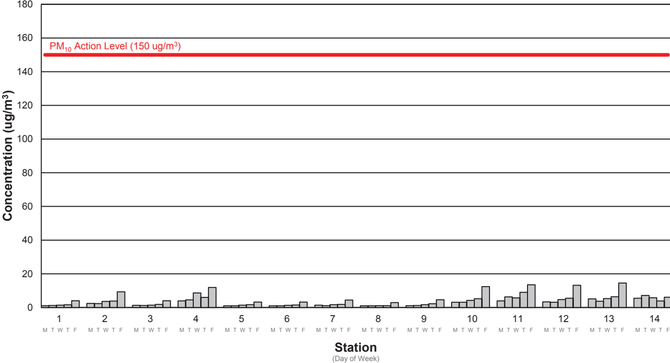
Average PM10 Concentration Week 171: 2/19/2024 - 2/23/2024
