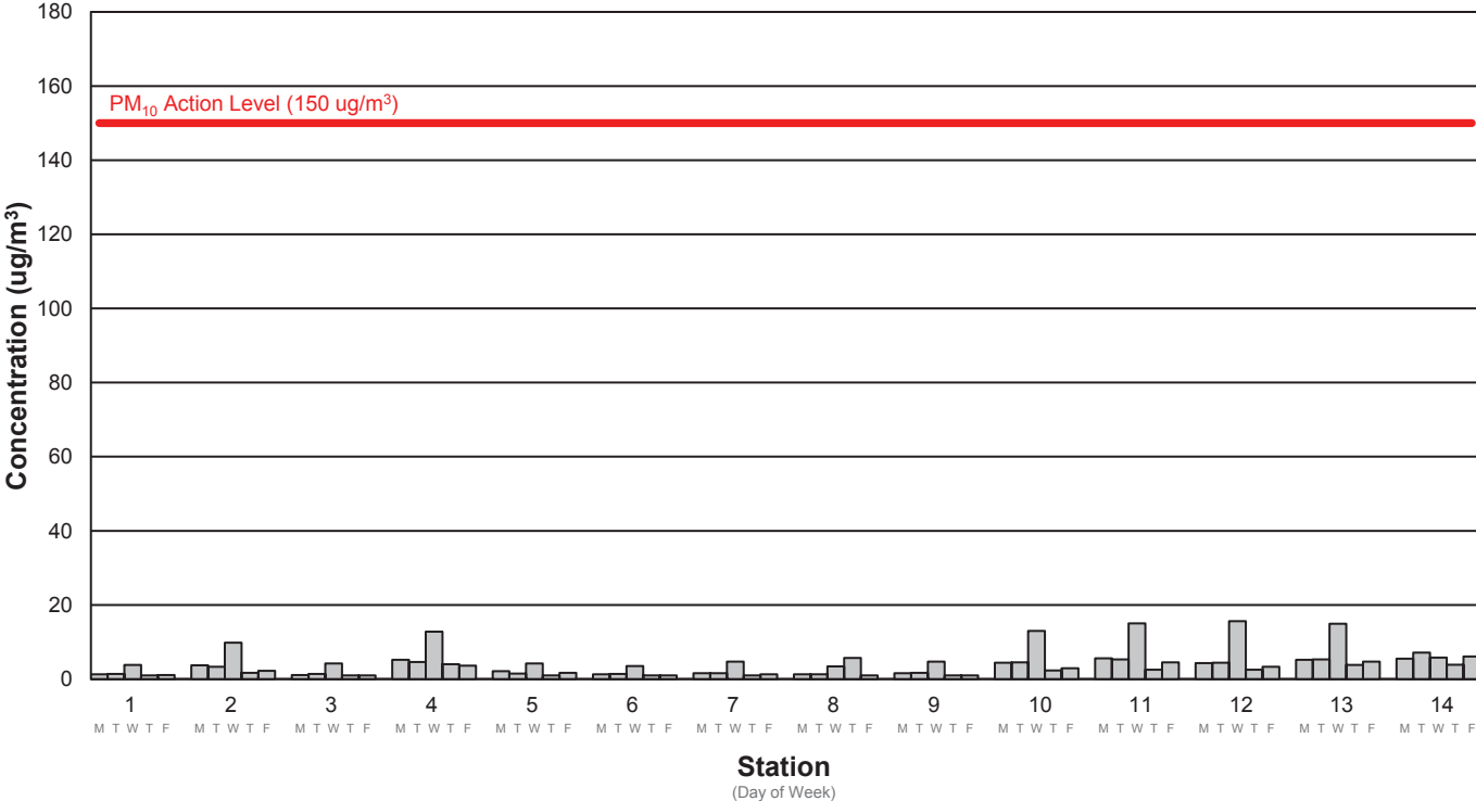
Average PM10 Concentration Week 173: 3/4/2024 - 3/8/2024
