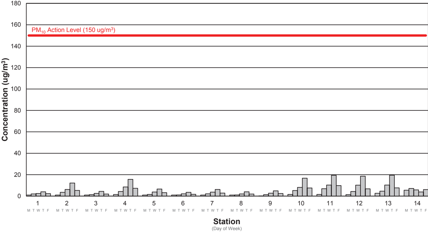
Average PM10 Concentration Week 174: 3/11/2024 - 3/15/2024
