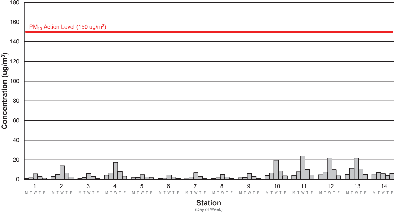
Average PM10 Concentration Week 176: 3/25/2024 - 3/29/2024
