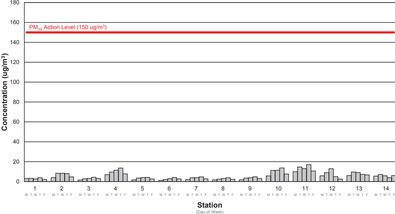
Average PM10 Concentration Week 178: 4/8/2024 - 4/12/2024
