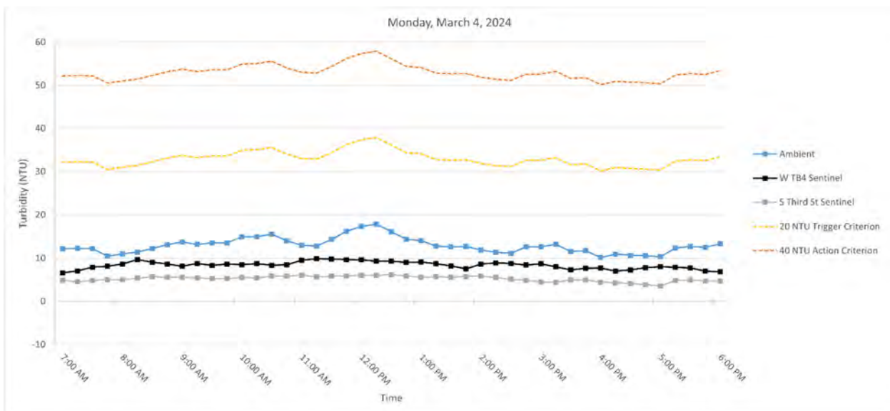
Figure 3. Hourly rolling average turbidity readings on Monday, March 4, 2024, from 7 AM to 6 PM.
