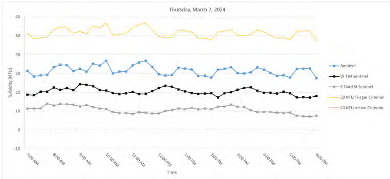
Figure 5. Hourly rolling average turbidity readings on Thursday, March 7, 2024, from 7 AM to 6 PM.
