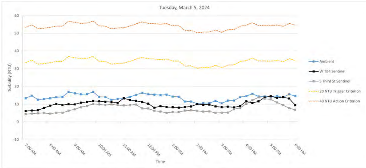
Figure 3. Hourly rolling average turbidity readings on Tuesday, March 5, 2024, from 7 AM to 6 PM.
