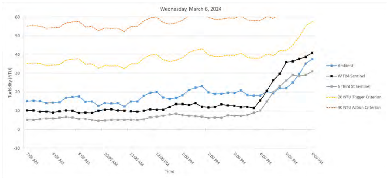
Figure 4. Hourly rolling average turbidity readings on Wednesday, March 6, 2024, from 7 AM to 6 PM.
