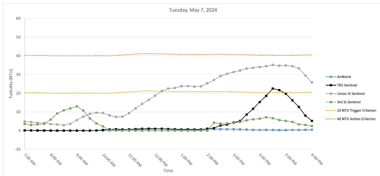
Figure 3. Hourly rolling average turbidity readings on Tuesday, May 7, 2024, from 7 AM to 6 PM.
