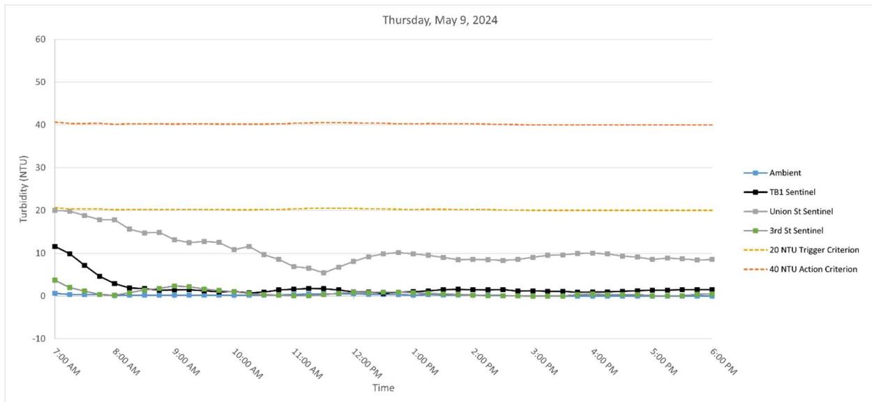
Figure 5. Hourly rolling average turbidity readings on Thursday, May 9, 2024, from 7 AM to 6 PM.
