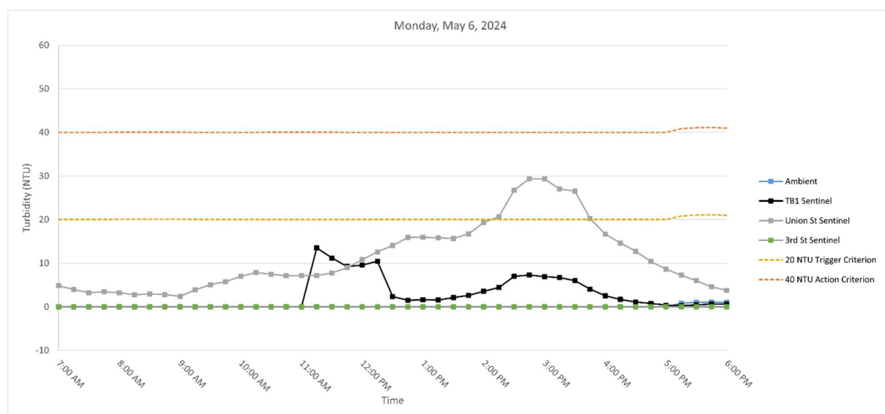
Figure 3. Hourly rolling average turbidity readings on Monday, May 6, 2024, from 7 AM to 6 PM.
