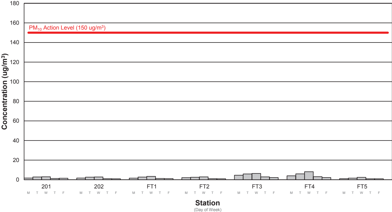
Average PM10 Concentration Week 189: 6/24/2024 - 6/28/2024
