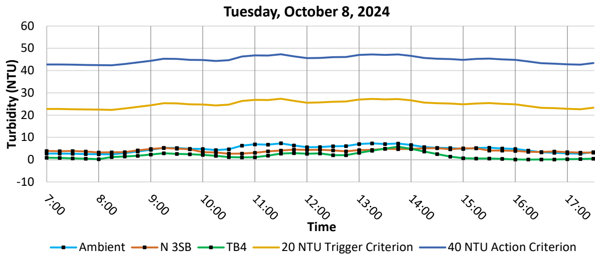
Figure 4. Hourly rolling average turbidity readings from 07:00 to 17:30
