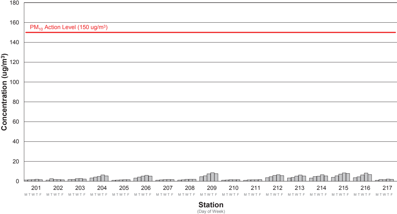
Average PM10 Concentration Week 16: 9/30/2024 - 10/4/2024
