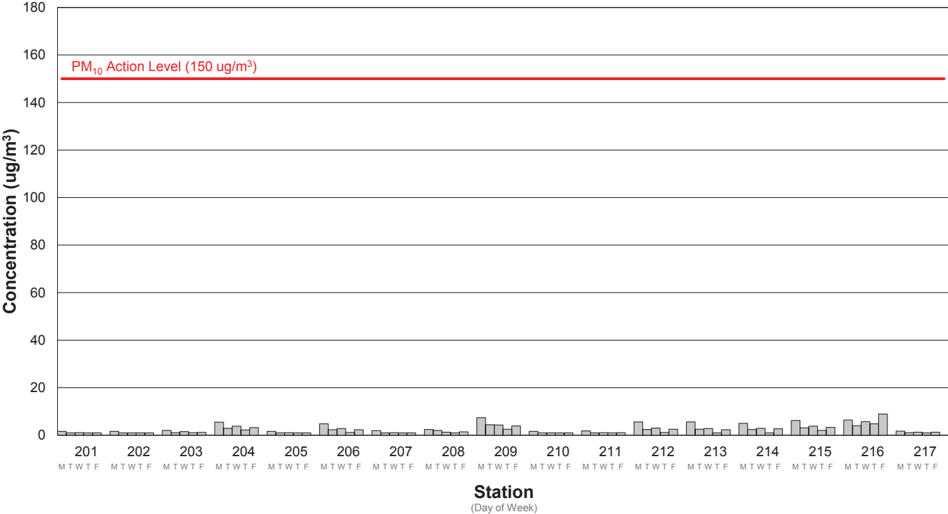
Average PM10 Concentration Week 17: 10/7/2024 - 10/11/2024
