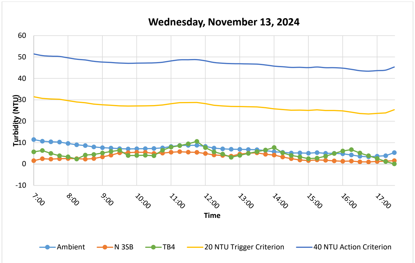
Figure 4. Hourly rolling average turbidity readings from 07:00 to 17:30.
