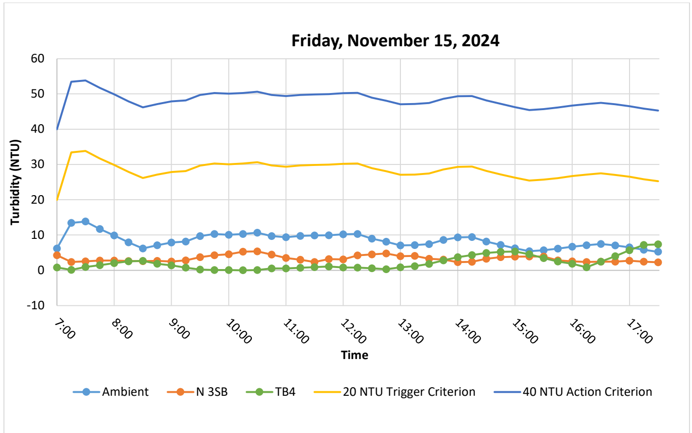
Figure 6. Hourly rolling average turbidity readings from 07:00 to 17:30.
