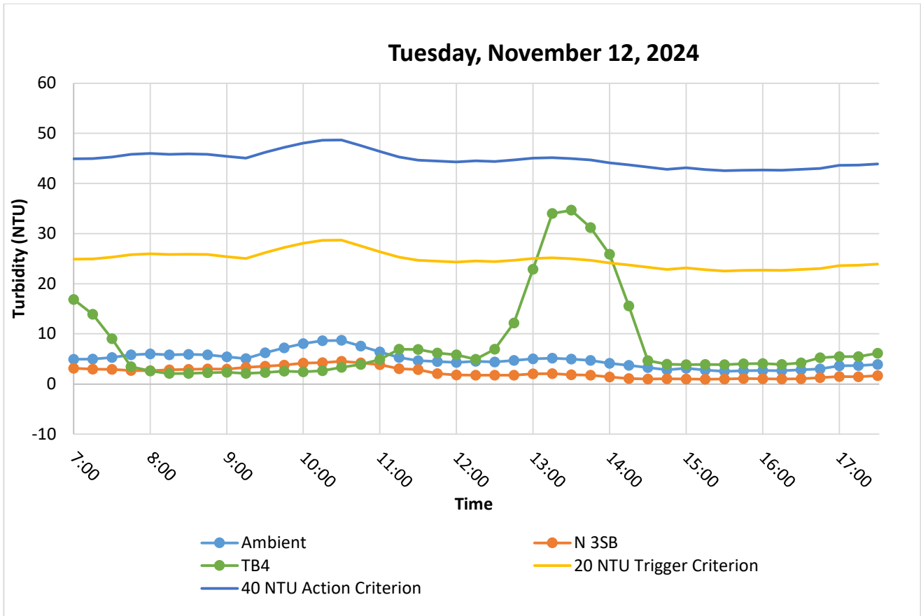
Figure 3. Hourly rolling average turbidity readings from 07:00 to 17:30. Exceedance to trigger action due to prop wash near TB4 sonde due to vessel movement within 100-feet of the monitoring location.
