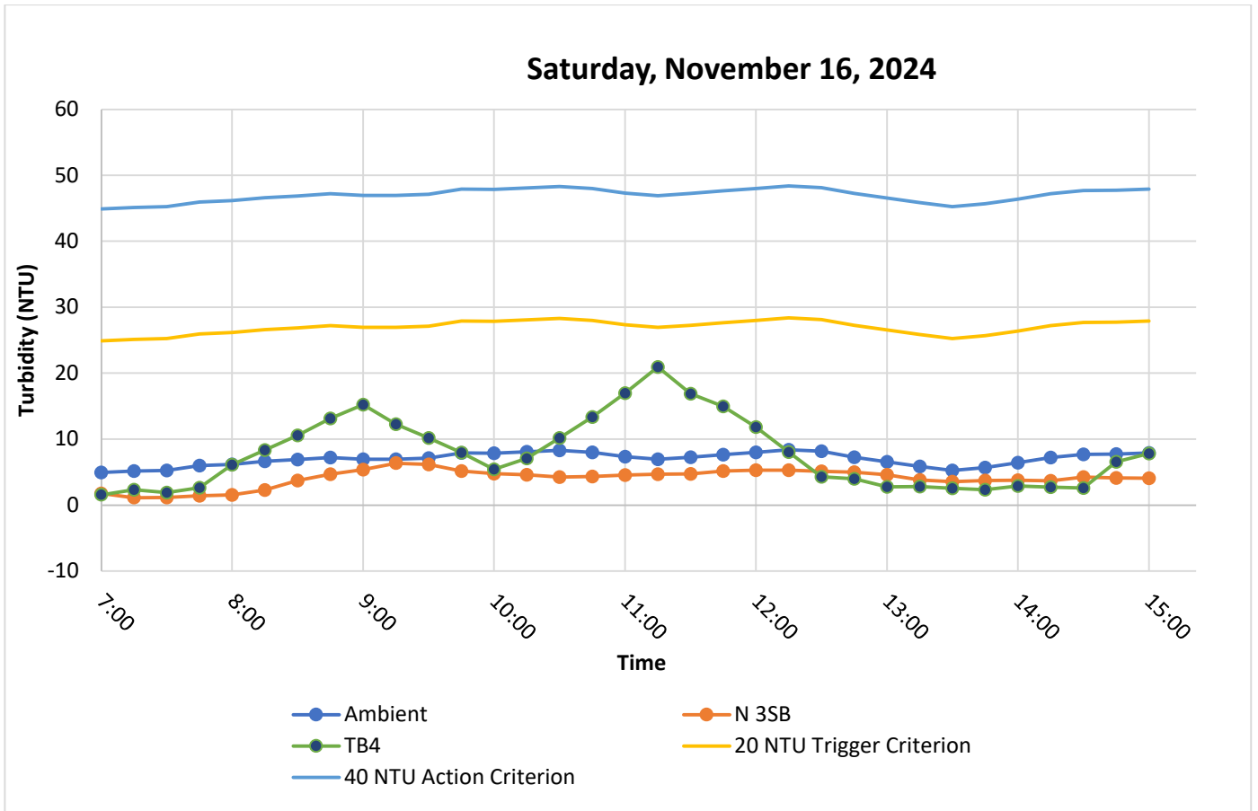
Figure 7. Hourly rolling average turbidity readings from 07:00 to 15:00.
