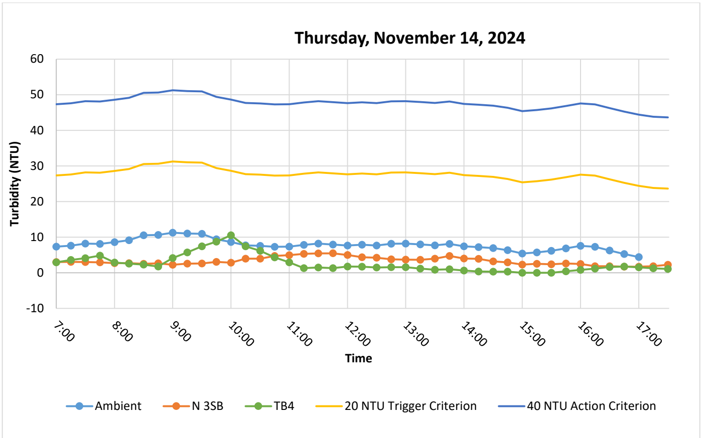
Figure 5. Hourly rolling average turbidity readings from 07:00 to 17:30.
