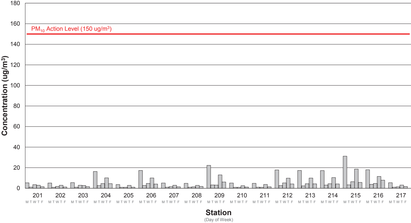
Average PM10 Concentration Week 42: 3/31/2025 - 4/4/2025
