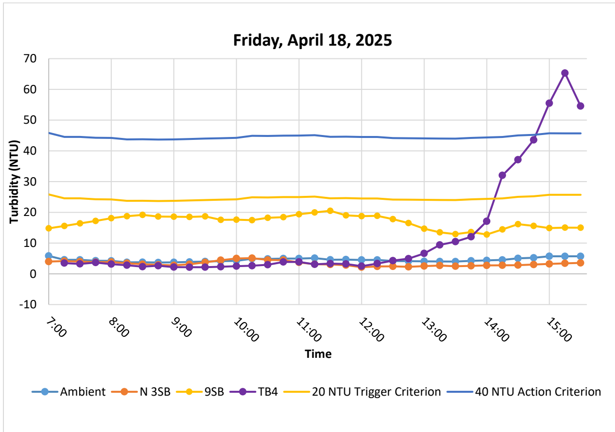
Figure 7. Hourly rolling average turbidity readings from 07:00 to 15:30. The elevated reading recorded by the TB4 sonde was unrelated to in-water construction activities. The TB4 sonde experienced a signal outage at the start of the day resulting in data not being reported at 07:00.
