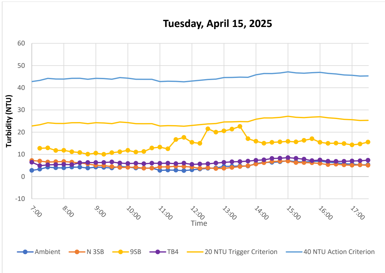
Figure 4. Hourly rolling average turbidity readings from 07:00 to 17:30. The 9SB sonde experienced a signal outage at the start of the day resulting in data not being reported at 07:00.
