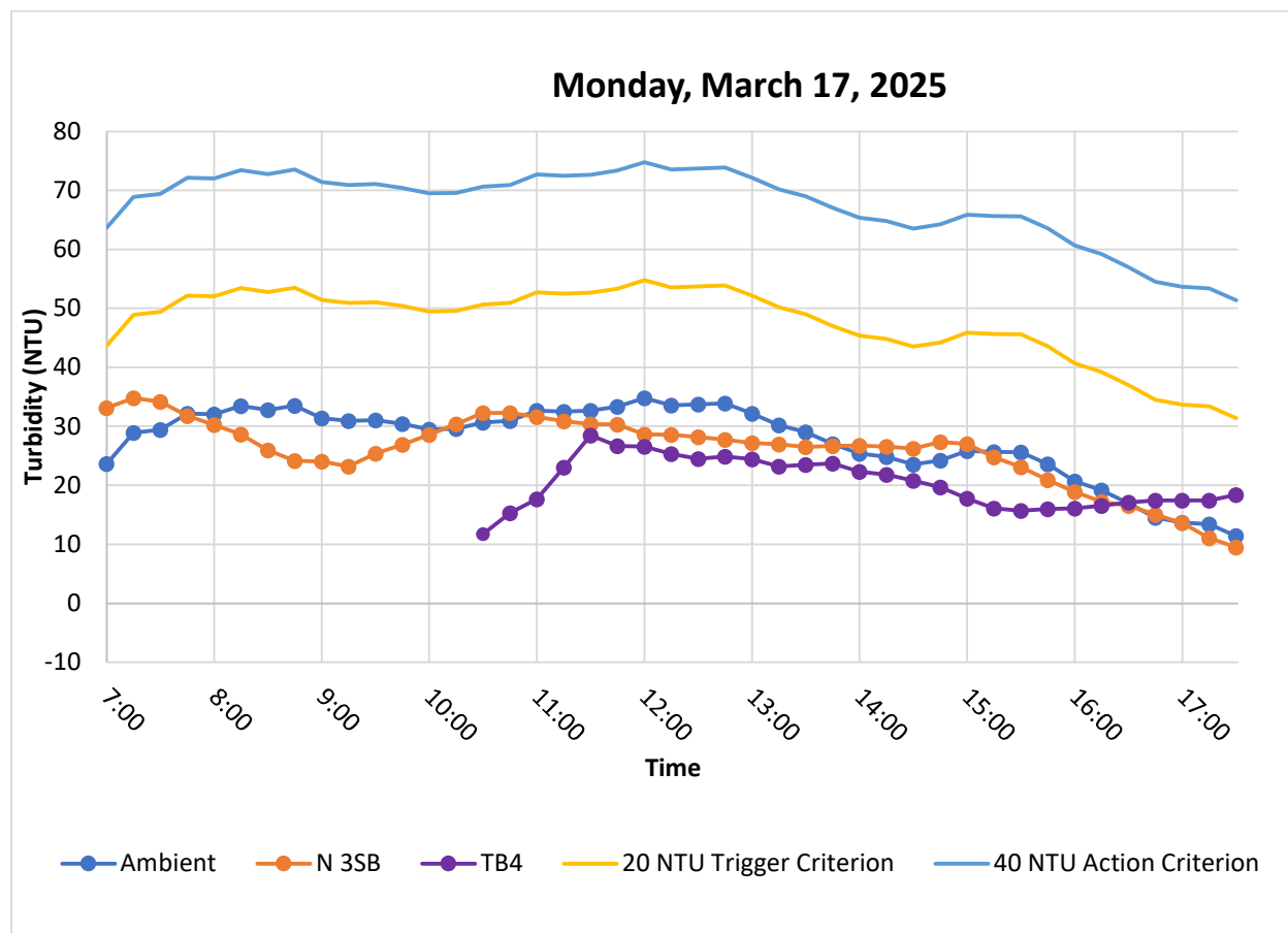
Figure 3. Hourly rolling average turbidity readings from 07:00 to 17:30. The TB4 sonde was deployed at 10:30 AM.
