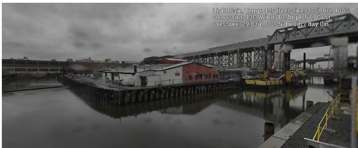
Figure 8 – April 7, 2025. General Conditions in Canal north of 9 th Street Bridge near TB6 during in-waterway construction activities.
