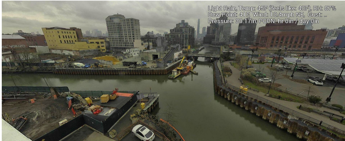
Figure 10 – April 11, 2025. General Conditions in Canal south of 3 rd Street Bridge near TB4 during in-waterway construction activities.
