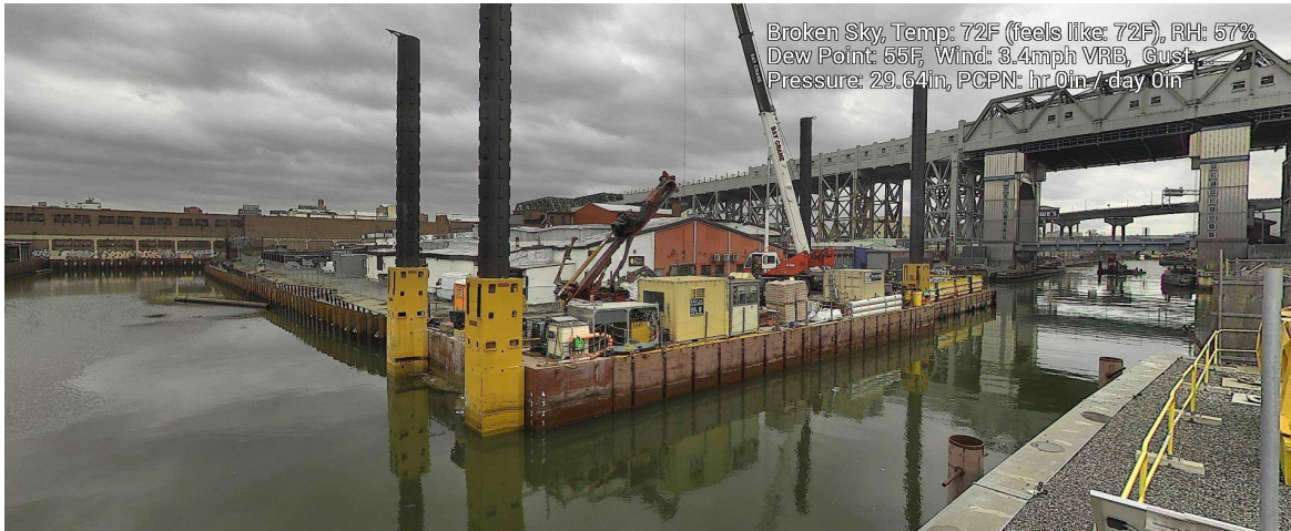
Figure 8 – March 31, 2025. General Conditions in Canal north of 9 th Street Bridge near TB6 during in-waterway construction activities.
