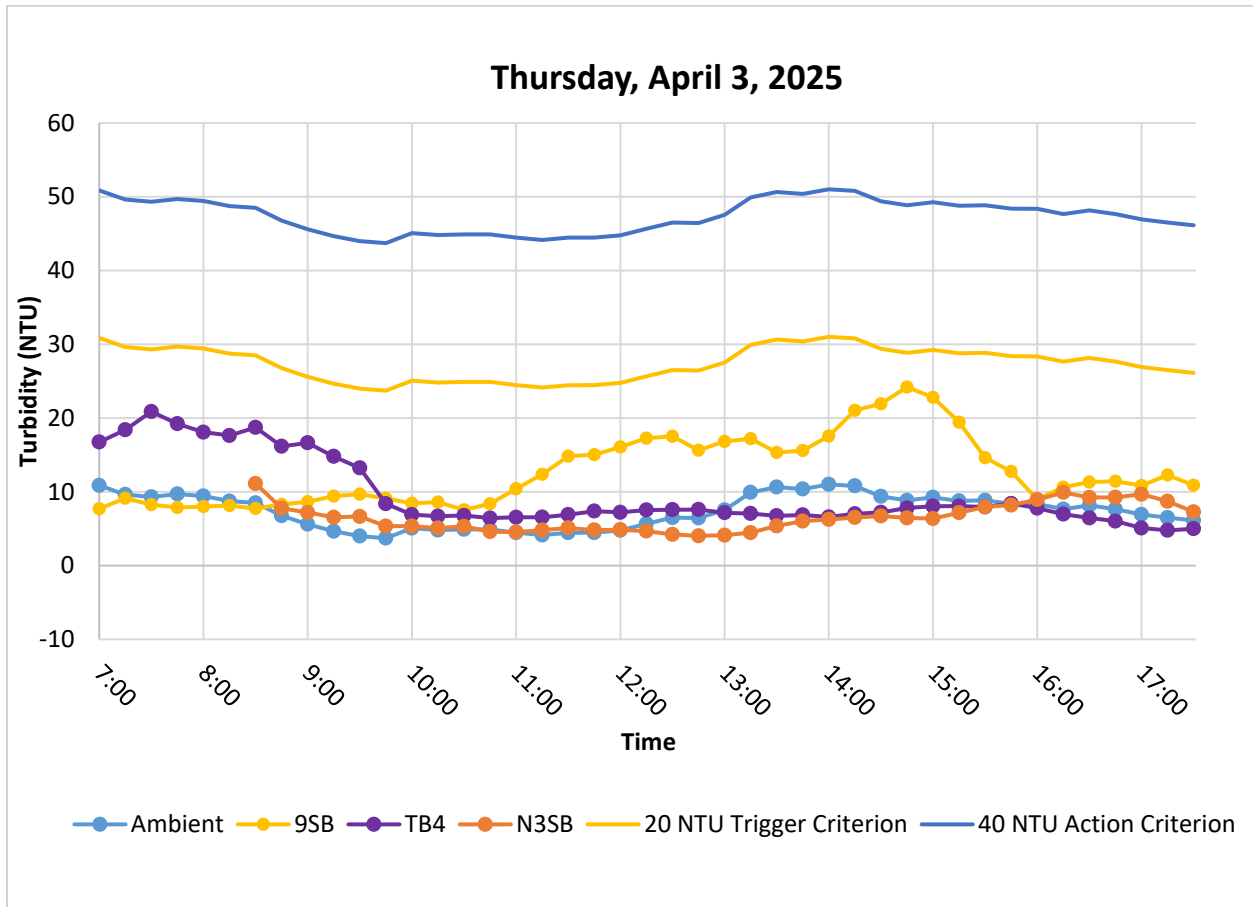
Figure 6. Hourly rolling average turbidity readings from 07:00 to 17:30. The N3SB sonde was deployed and began reporting data at 08:30.
