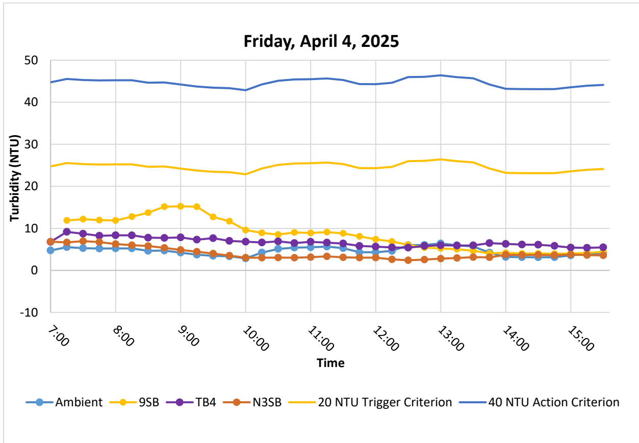
Figure 7. Hourly rolling average turbidity readings from 07:00 to 15:30. The 9SB sonde experienced a signal outage at the start of the day resulting in data not being reported at 07:00.
