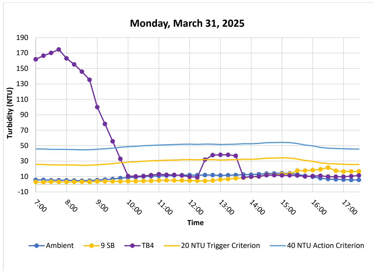
Figure 3. Hourly rolling average turbidity readings from 07:00 to 17:30. The elevated readings recorded by the TB4 sonde were unrelated to in-water construction activities.
