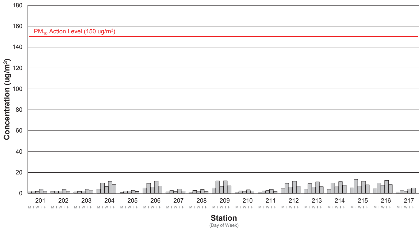
Average PM10 Concentration Week 45: 4/21/2025 - 4/25/2025
