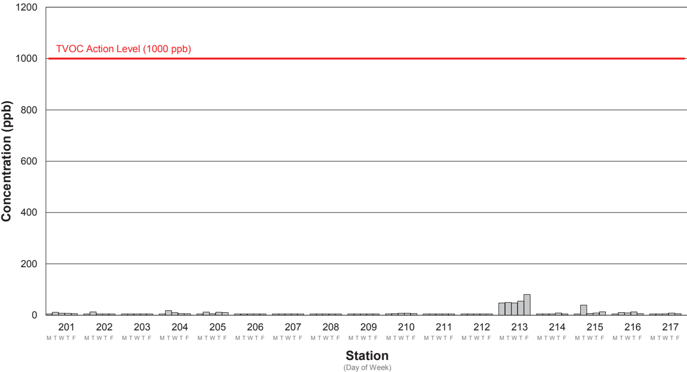
Average TVOC Concentration Week 45: 4/21/2025 - 4/25/2025
