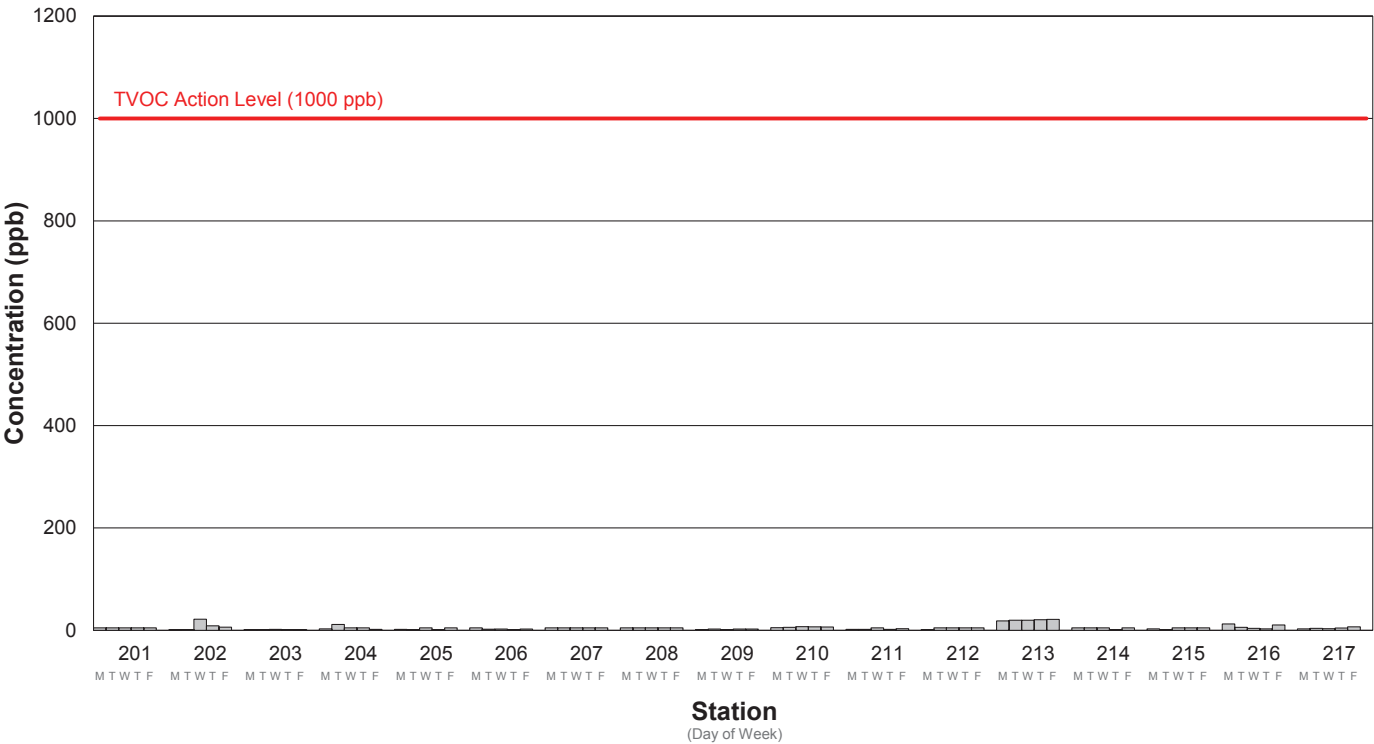
Average TVOC Concentration Week 49: 5/19/2025 - 5/23/2025
