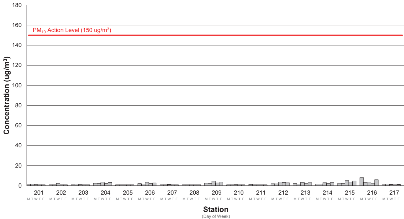
Average PM10 Concentration Week 49: 5/19/2025 - 5/23/2025
