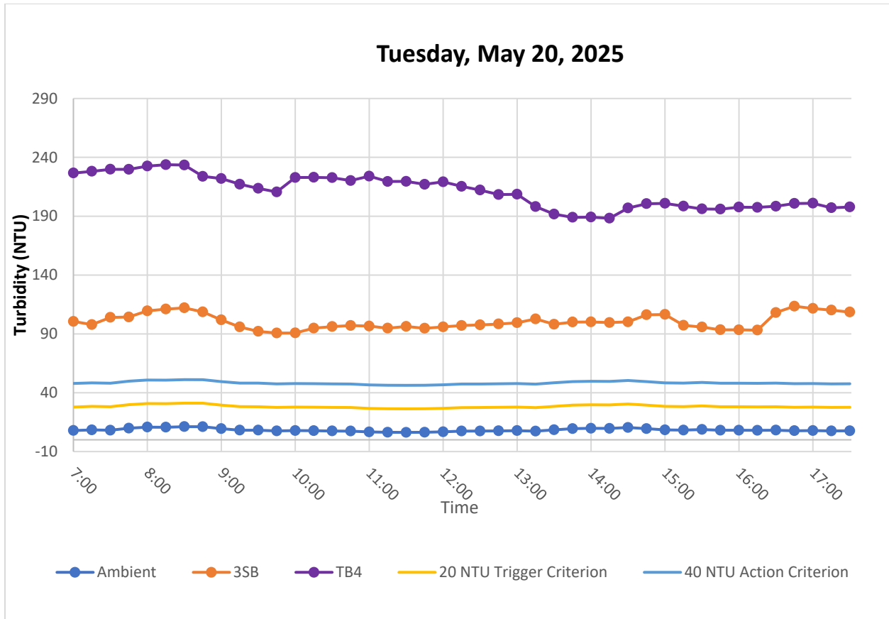
Figure 4. Hourly rolling average turbidity readings from 07:00 to 17:30. The elevated readings recorded by the TB4 and 3SB sondes were unrelated to in-water construction activities. 9SB was removed from service due to telemetry failure and no readings were reported for this day.
