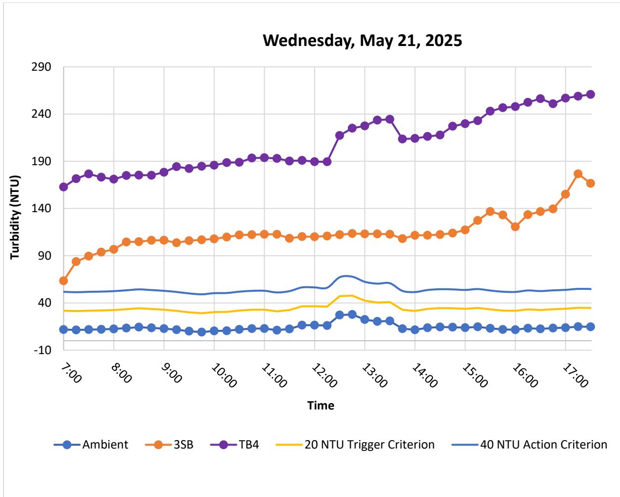
Figure 5. Hourly rolling average turbidity readings from 07:00 to 17:30. The elevated readings recorded by the TB4 and 3SB sondes were unrelated to in-water construction activities. 9SB was removed from service due to telemetry failure and no readings were reported for this day.
