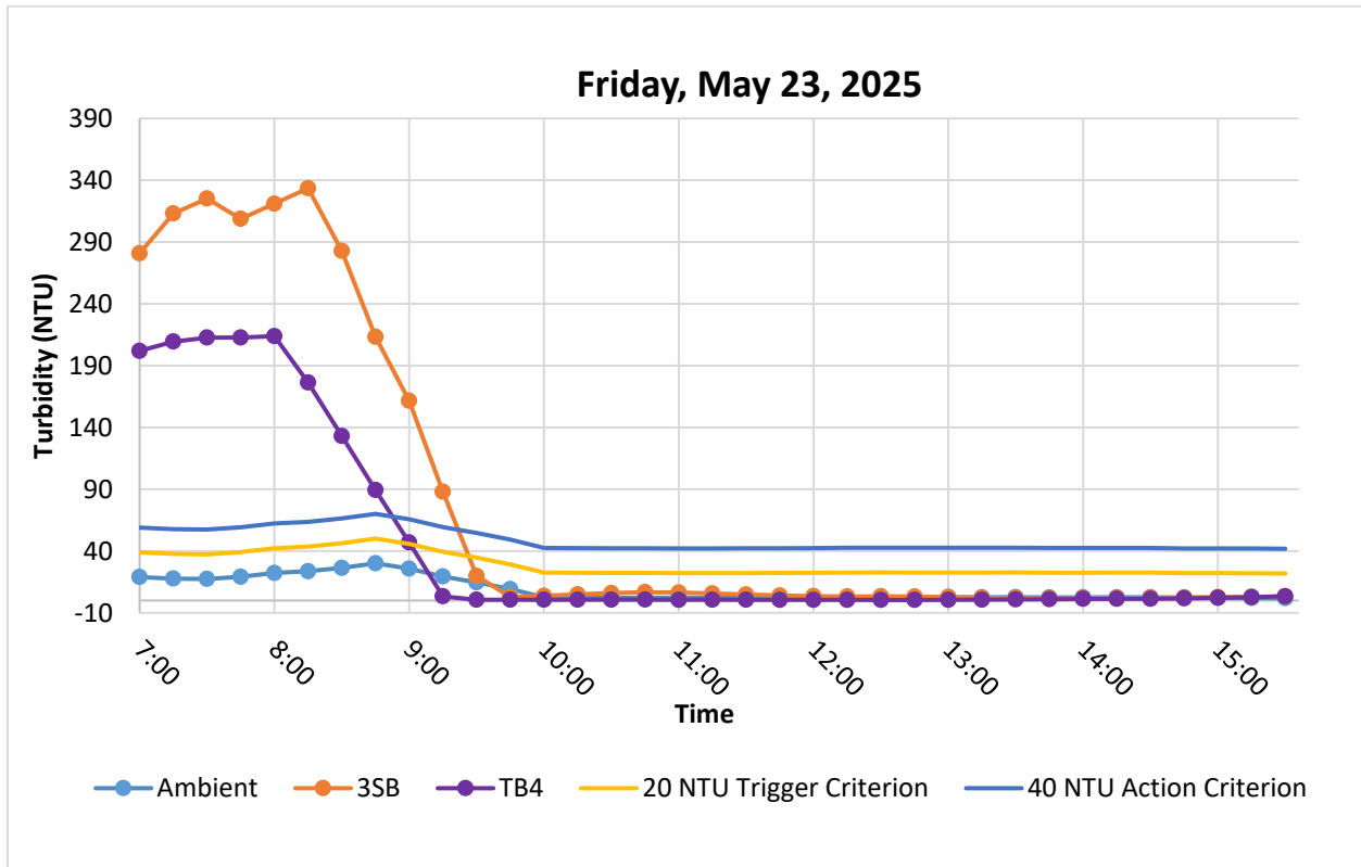
Figure 7. Hourly rolling average turbidity readings from 07:00 to 15:30. The elevated readings recorded by the TB4 and 3SB sondes were unrelated to in-water construction activities. 9SB was removed from service due to telemetry failure and no readings were reported for this day.
