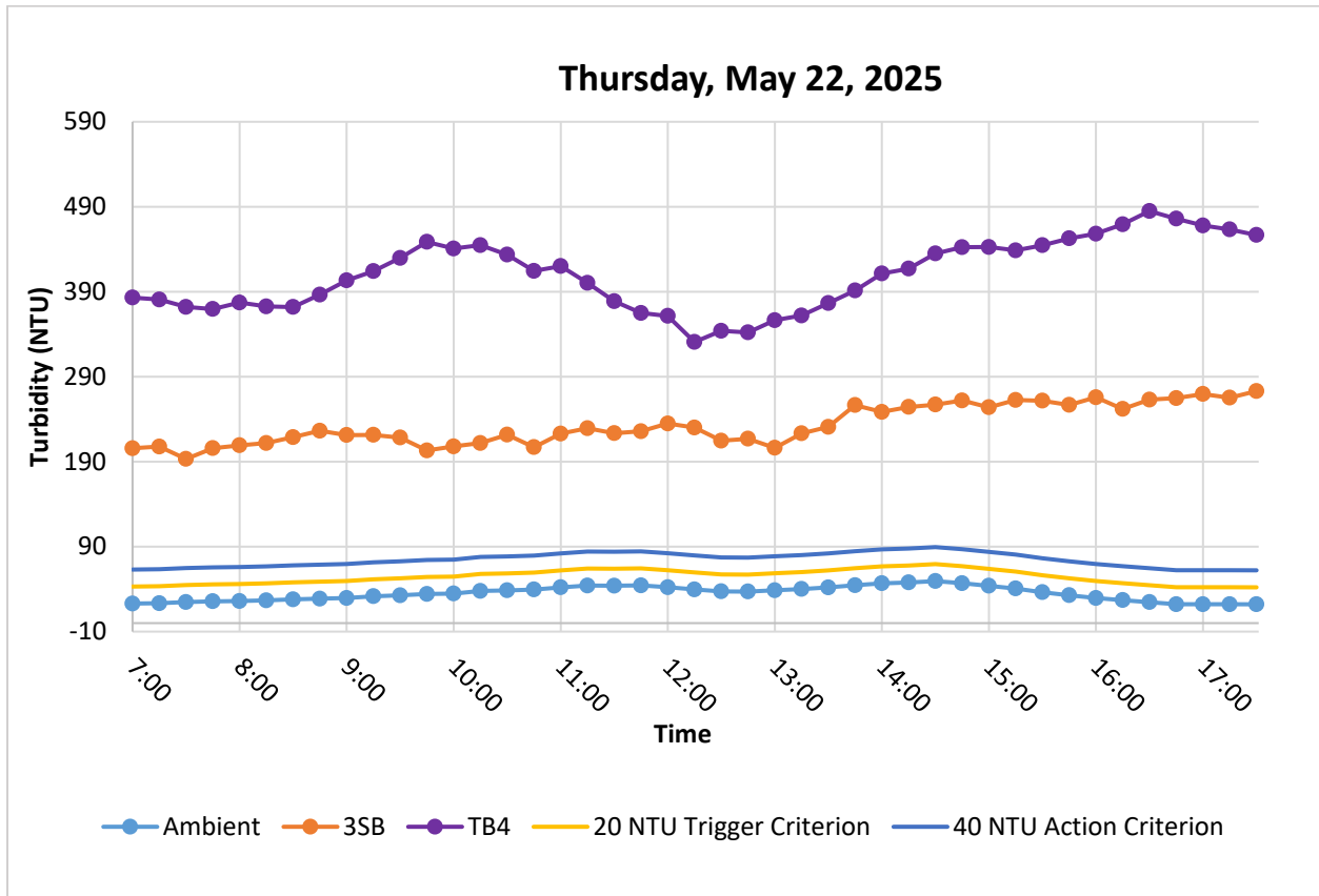
Figure 6. Hourly rolling average turbidity readings from 07:00 to 17:30. The elevated readings recorded by the TB4 and 3SB sondes were unrelated to in-water construction activities. 9SB was removed from service due to telemetry failure and no readings were reported for this day.
