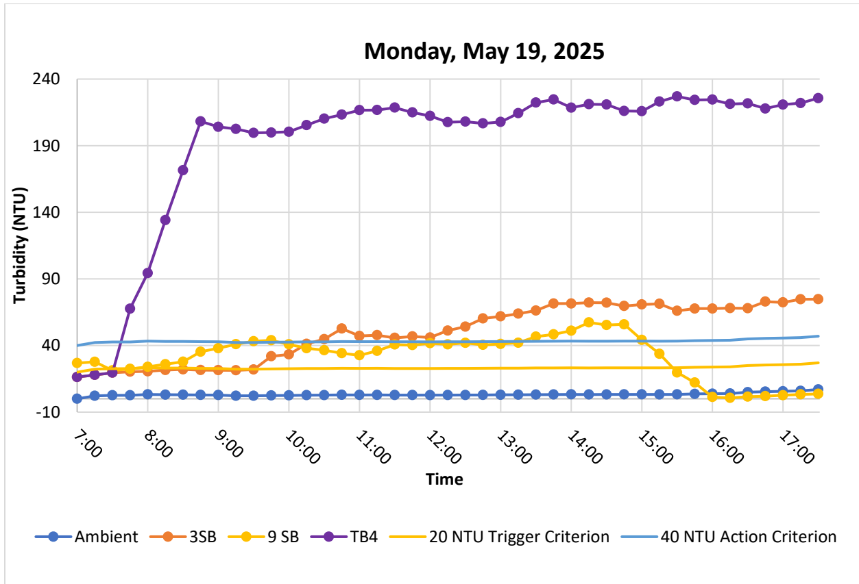
Figure 3. Hourly rolling average turbidity readings from 07:00 to 17:30. The elevated readings recorded by the TB4, 9SB, and 3SB sondes were unrelated to in-water construction activities.
