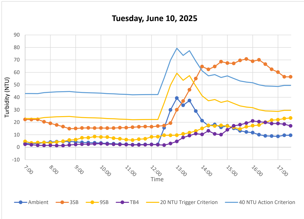
Figure 4. Hourly rolling average turbidity readings from 07:00 to 17:30. The elevated readings recorded by the 3SB sonde were unrelated to in-water construction activities.
