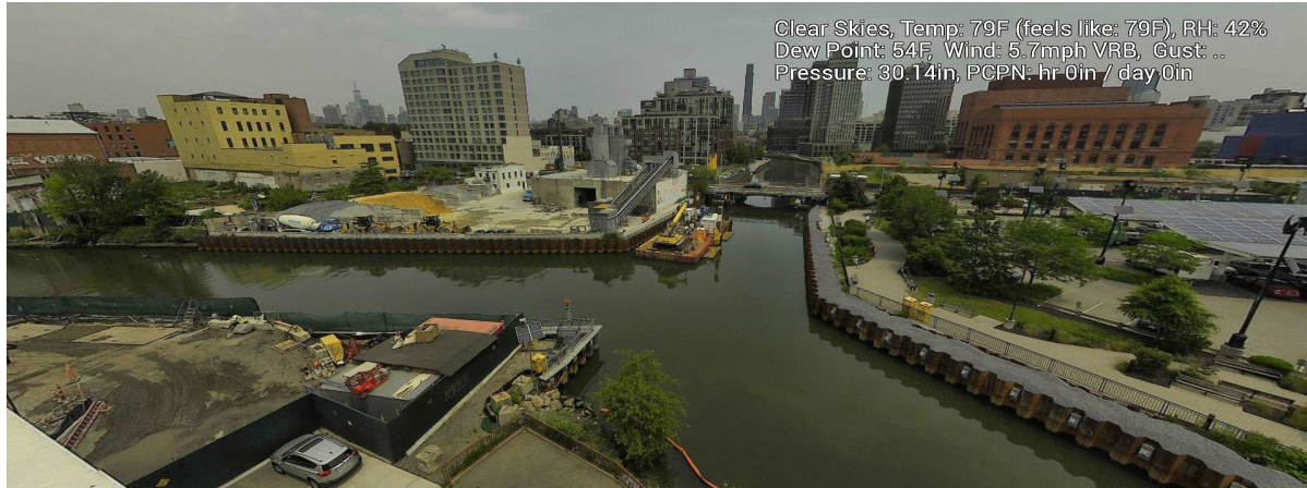
Figure 10 – June 13, 2025. General Conditions in Canal south of 3 rd Street Bridge near TB4 during in-waterway construction activities.
