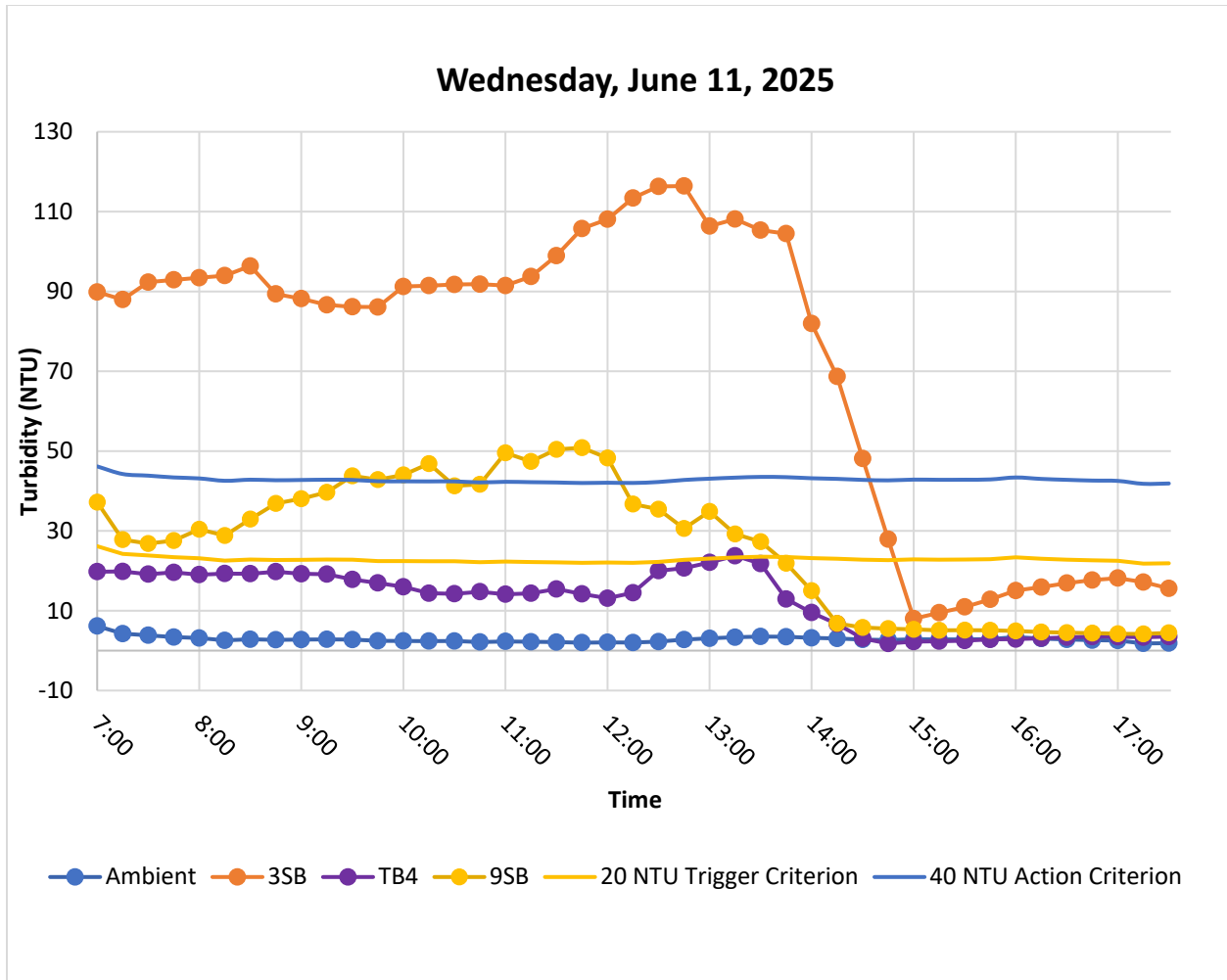
Figure 5. Hourly rolling average turbidity readings from 07:00 to 17:30. The elevated readings recorded by the 3SB, 9SB, and TB4 sonde were unrelated to in-water construction activities.
