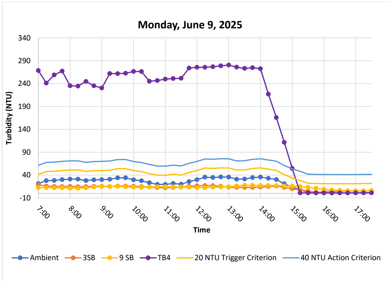
Figure 3. Hourly rolling average turbidity readings from 07:00 to 17:30. The elevated readings recorded by the TB4 sonde were unrelated to in-water construction activities.
