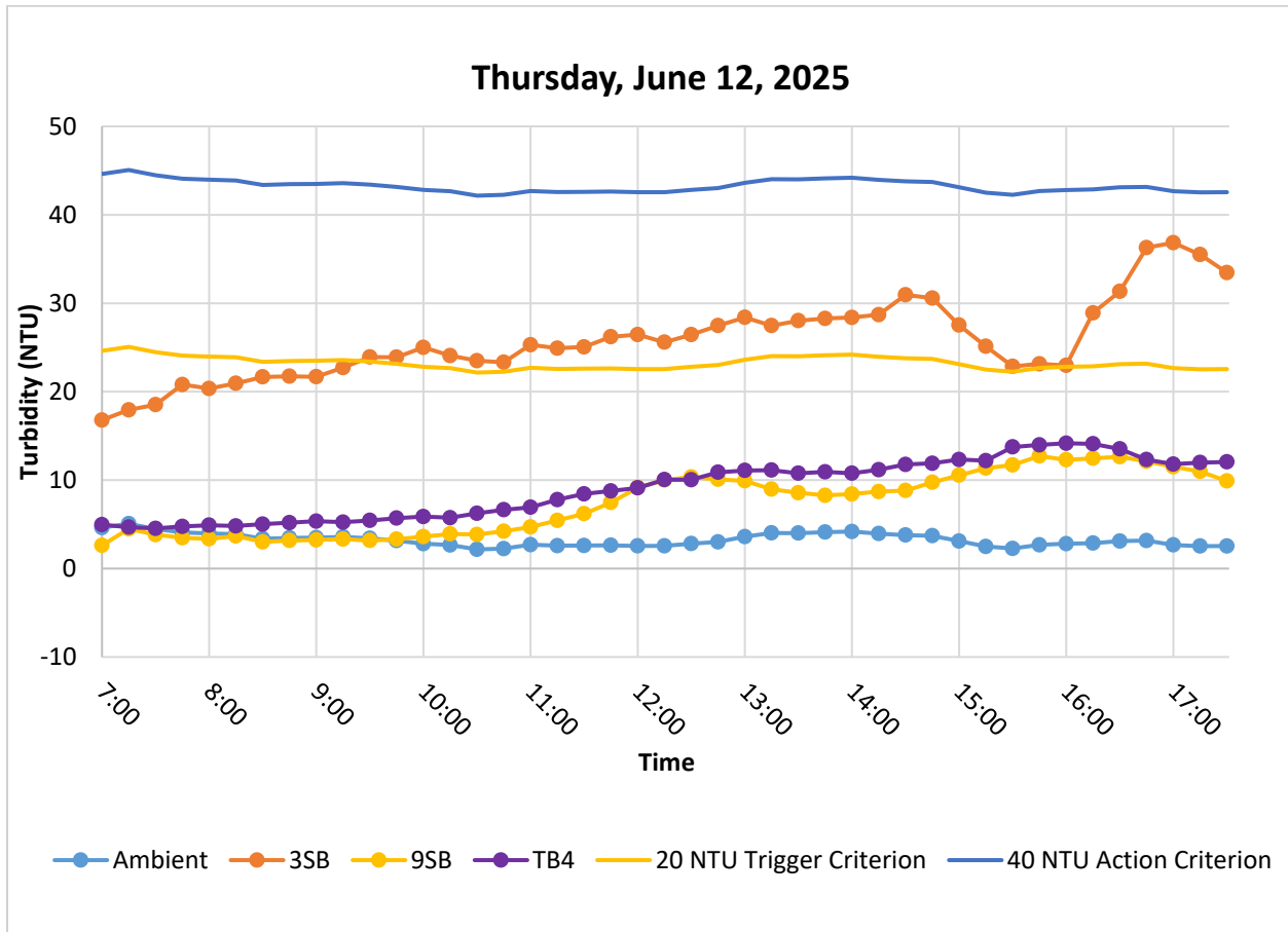
Figure 6. Hourly rolling average turbidity readings from 07:00 to 17:30. The elevated readings recorded by the 3SB sonde are unrelated to in-water construction activities.
