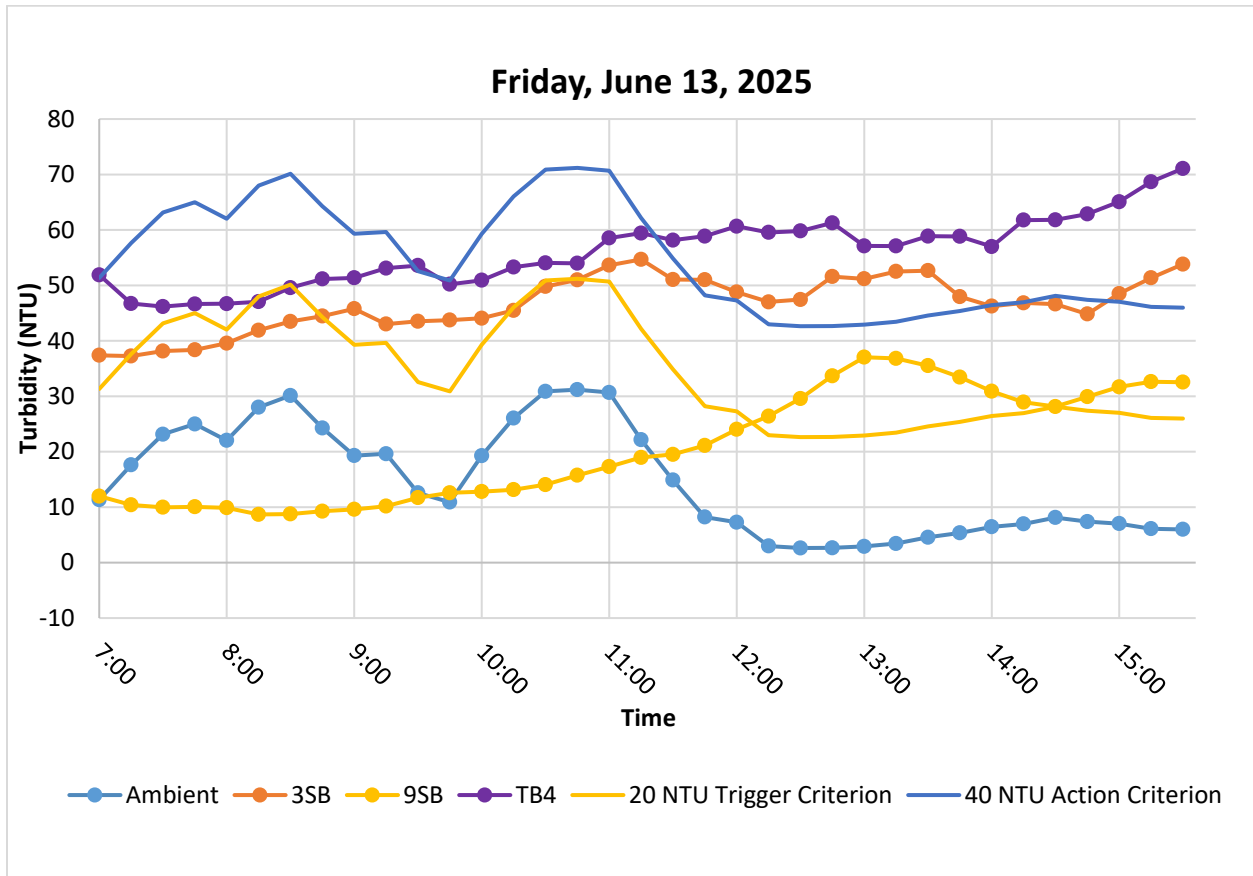
Figure 7. Hourly rolling average turbidity readings from 07:00 to 15:30. The elevated readings recorded by the 9SB, 3SB and TB4 sondes were unrelated to in-water construction activities.
