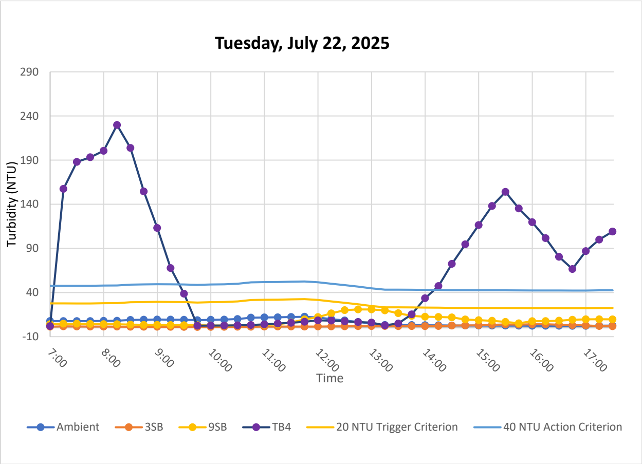
Figure 4. Hourly rolling average turbidity readings from 07:00 to 17:30. The elevated readings recorded by the TB4 sonde were unrelated to in-water construction activities
