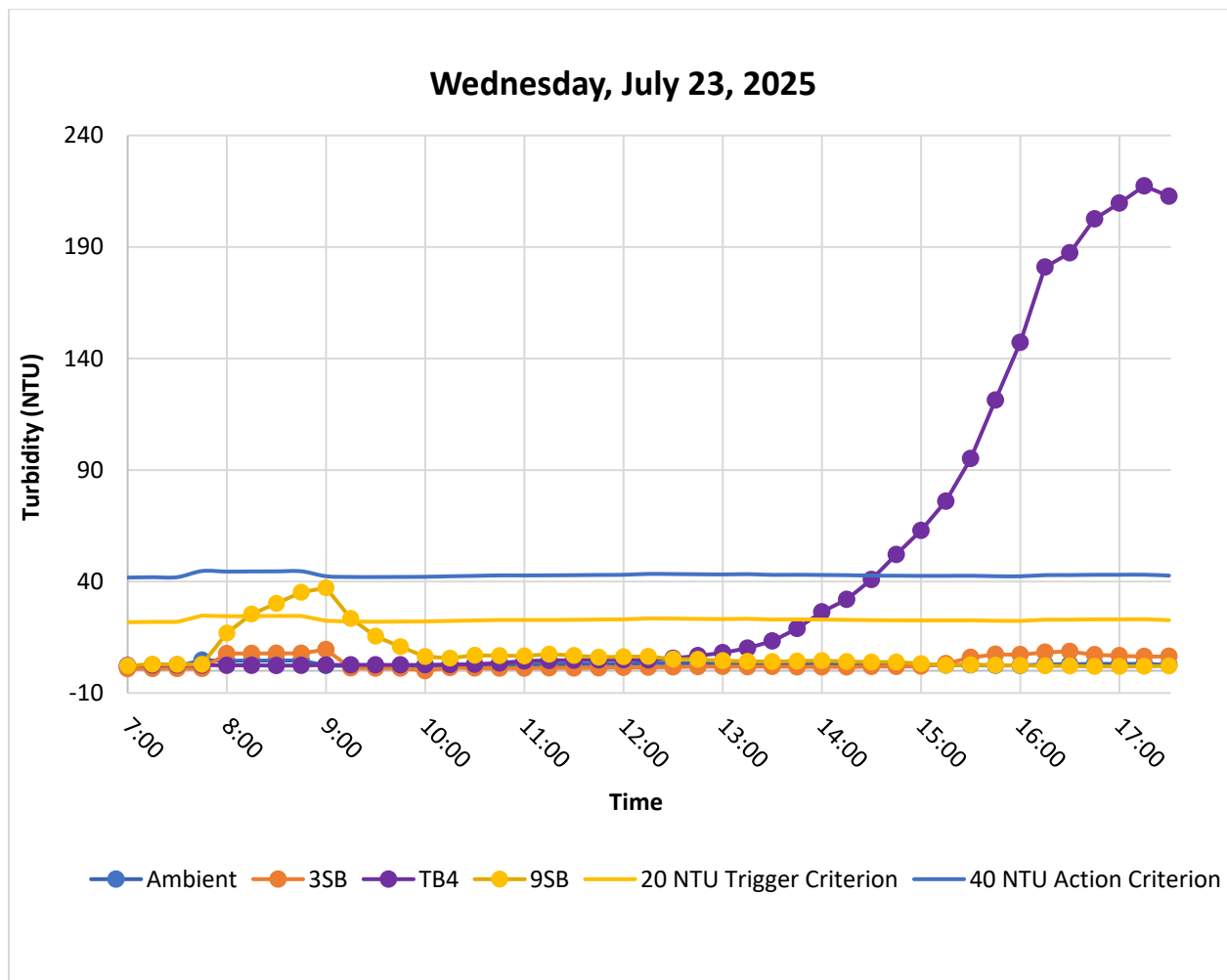
Figure 5. Hourly rolling average turbidity readings from 07:00 to 17:30. The elevated readings recorded by the TB4 and 9SB sondes were unrelated to in-water construction activities
