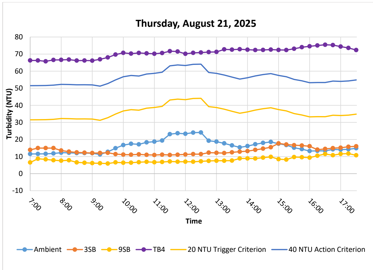
Figure 6. Hourly rolling average turbidity readings from 07:00 to 17:30. Elevated readings recorded by TB4 sonde were unrelated to in-water construction activities
