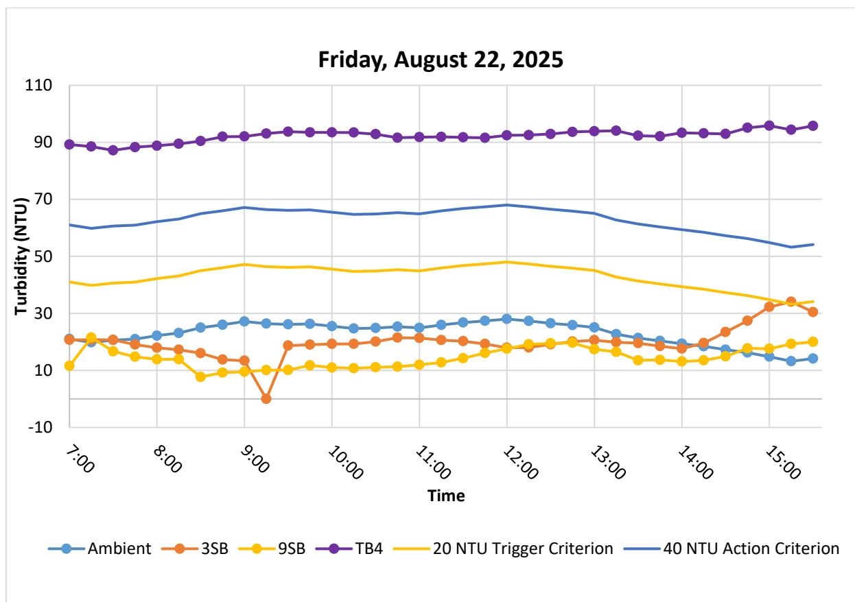
Figure 7. Hourly rolling average turbidity readings from 07:00 to 15:30. Elevated readings recorded by TB4 sonde were unrelated to in-water construction activities.
