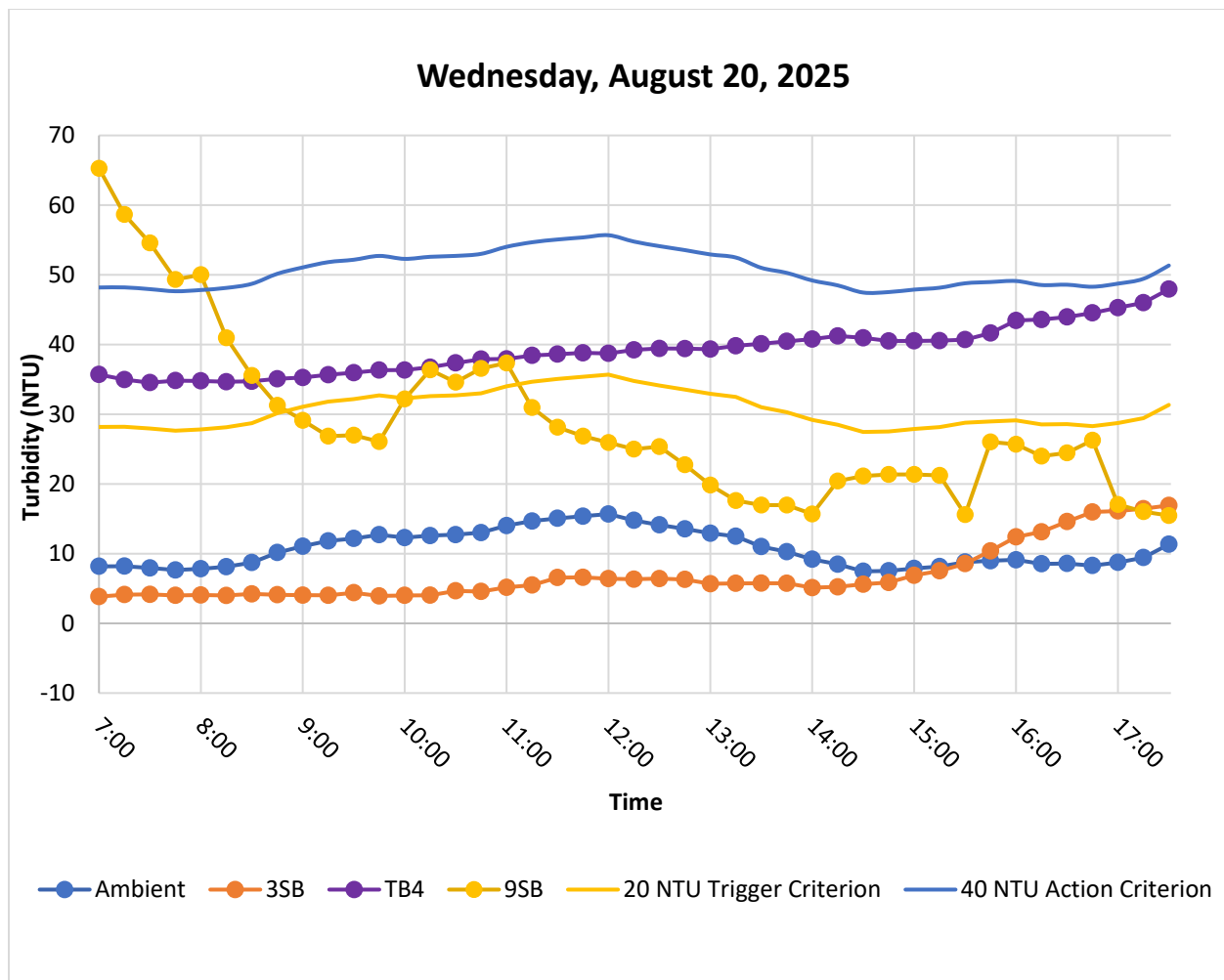
Figure 5. Hourly rolling average turbidity readings from 07:00 to 17:30. Elevated readings recorded by the 9SB and TB4 sondes were unrelated to in-water construction activities.
