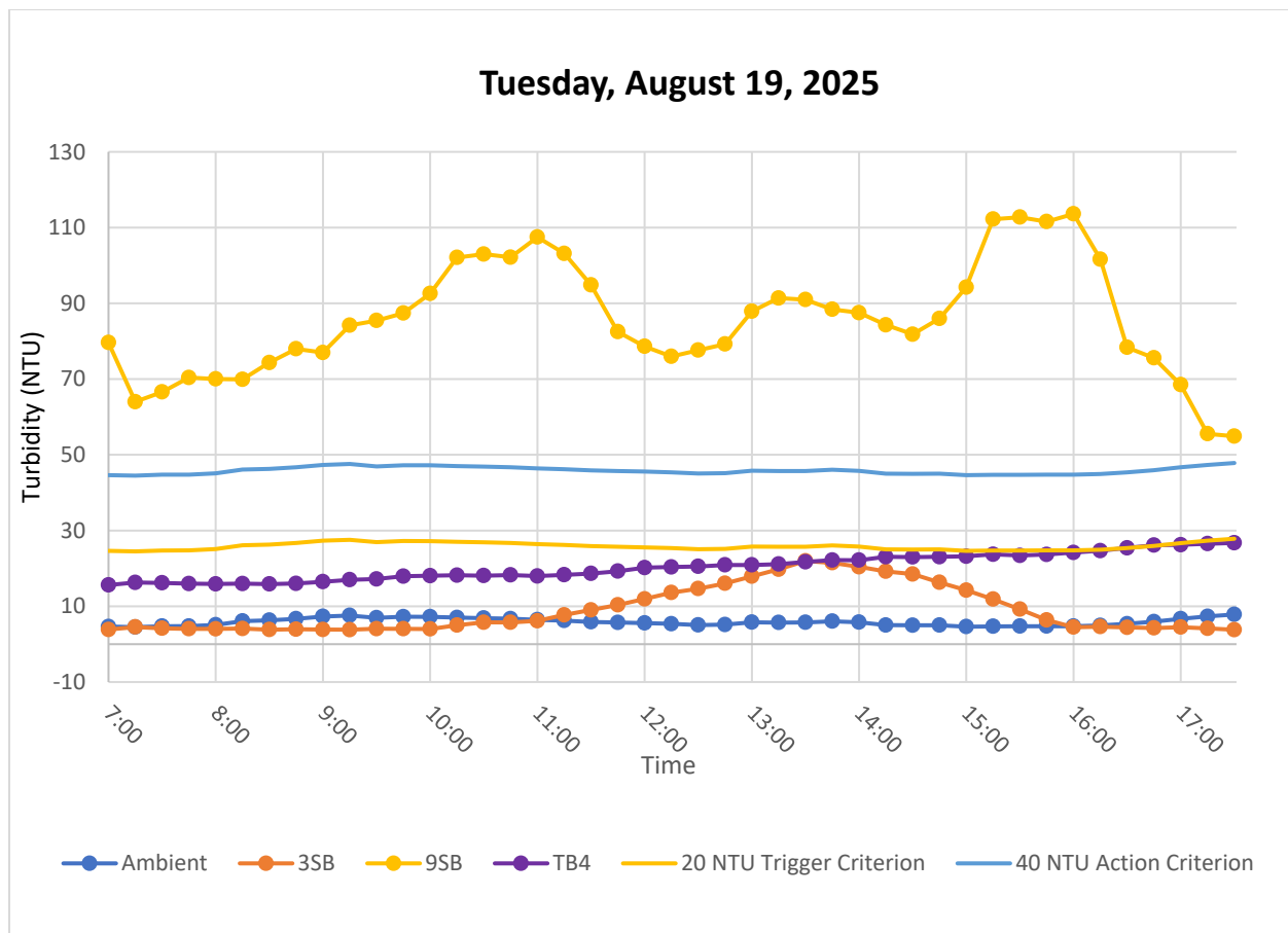
Figure 4. Hourly rolling average turbidity readings from 07:00 to 17:30. Elevated readings recorded by the 9SB and TB4 sondes were unrelated to in-water construction activities.
