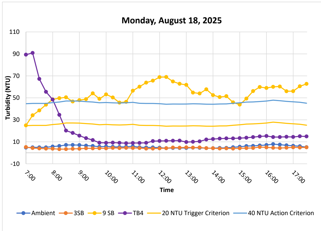
Figure 3. Hourly rolling average turbidity readings from 07:00 to 17:30. Elevated readings recorded by the 9SB and TB4 sondes were unrelated to in-water construction activities.
