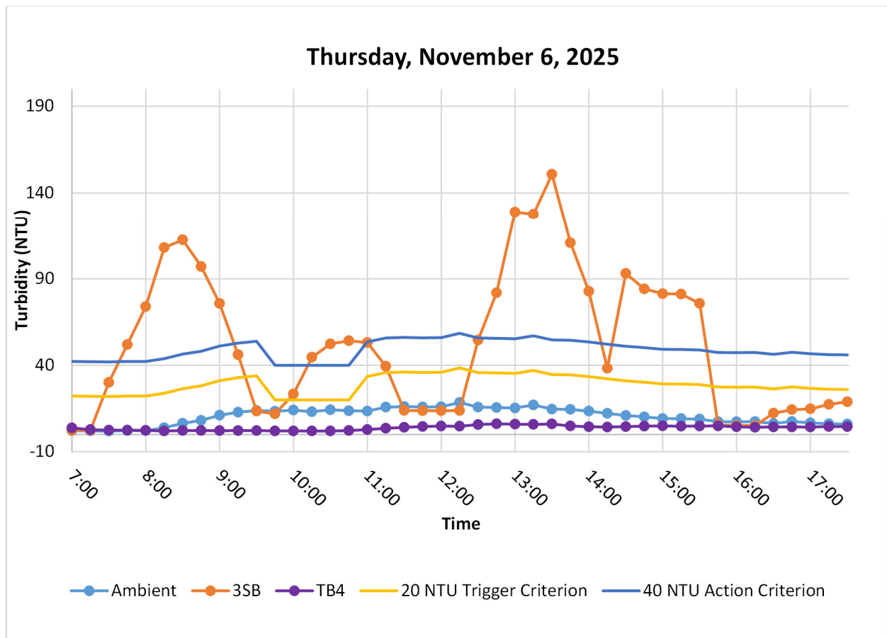
Figure 6. Hourly rolling average turbidity readings from 07:00 to 17:30. Elevated readings at 3SB are unrelated to in-water construction activities.
