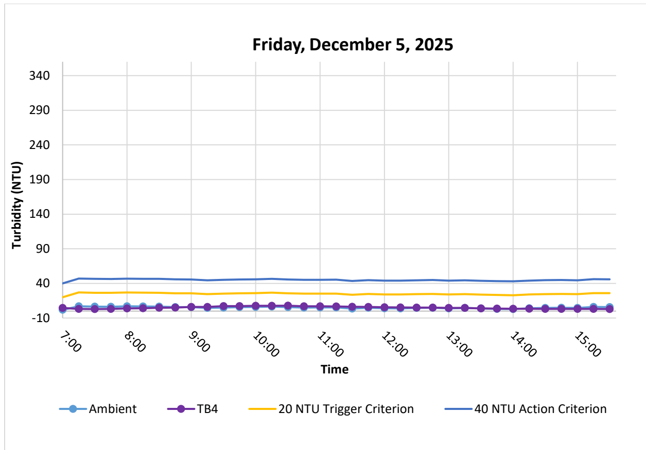
Figure 7. Hourly rolling average turbidity readings from 07:00 to 17:30.
