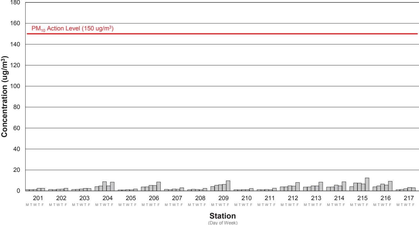
Average PM10 Concentration Week 64: 9/1/2025 - 9/5/2025
