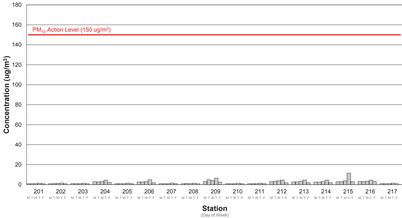
Average PM10 Concentration Week 72: 10/27/2025 - 10/31/2025
