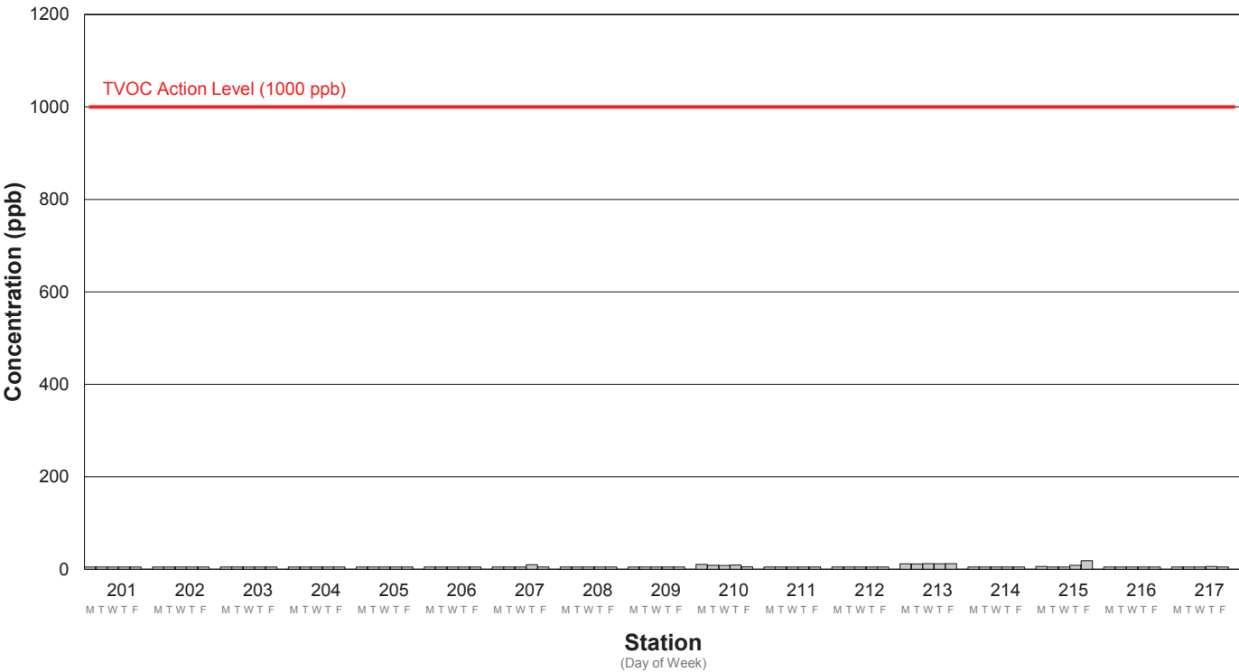
Average TVOC Concentration Week 72: 10/27/2025 - 10/31/2025
