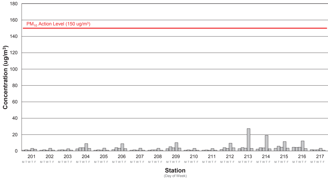
Average PM10 Concentration Week 77: 12/1/2025 - 12/5/2025
