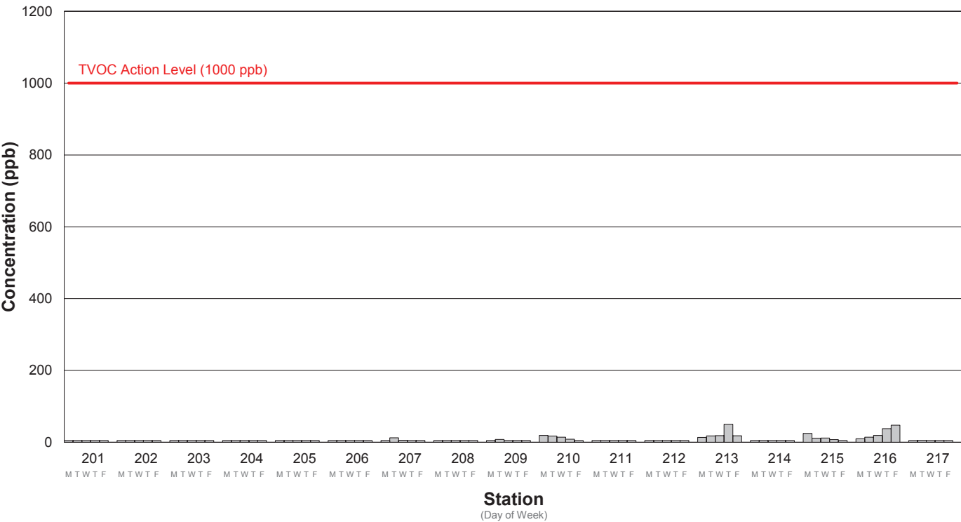
Average TVOC Concentration Week 77: 12/1/2025 - 12/5/2025
