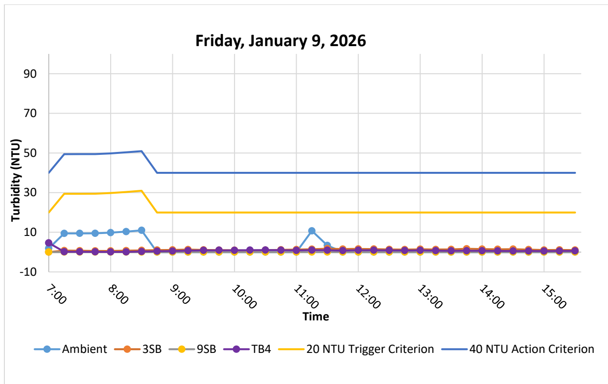
Figure 7. Hourly rolling average turbidity readings from 07:00 to 15:30. Elevated readings from the ambient buoy were excluded, with turbidity limits set at 20 and 40 NTU.
