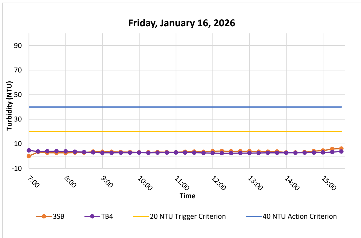
Figure 7. Hourly rolling average turbidity readings from 07:00 to 15:30. Elevated readings from the ambient buoy were excluded, with turbidity limits set at 20 and 40 NTU.
