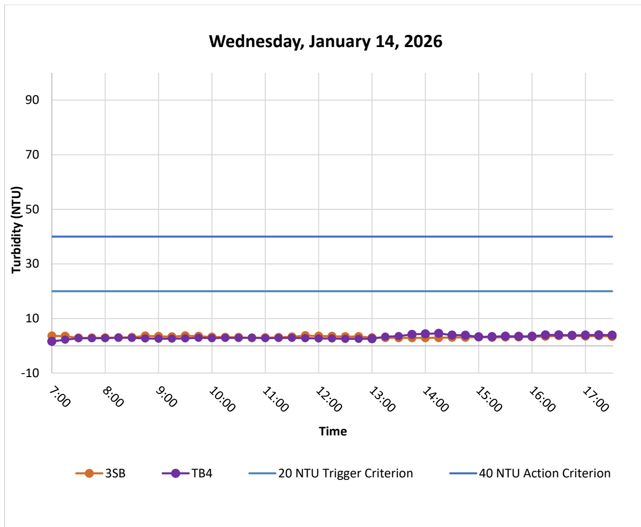
Figure 5. Hourly rolling average turbidity readings from 07:00 to 17:30. Elevated readings from the ambient buoy were excluded, with turbidity limits set at 20 and 40 NTU.
