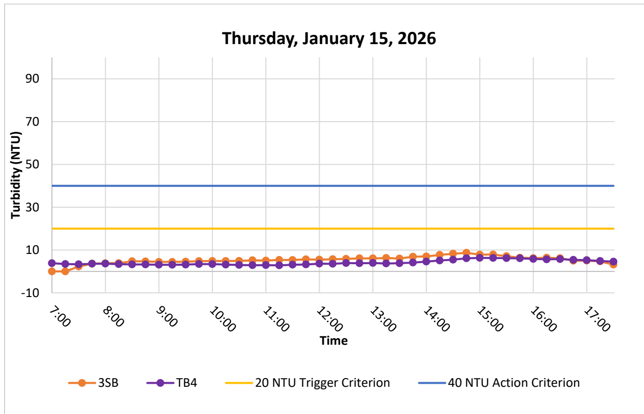
Figure 6. Hourly rolling average turbidity readings from 07:00 to 17:30. Elevated readings from the ambient buoy were excluded, with turbidity limits set at 20 and 40 NTU.
