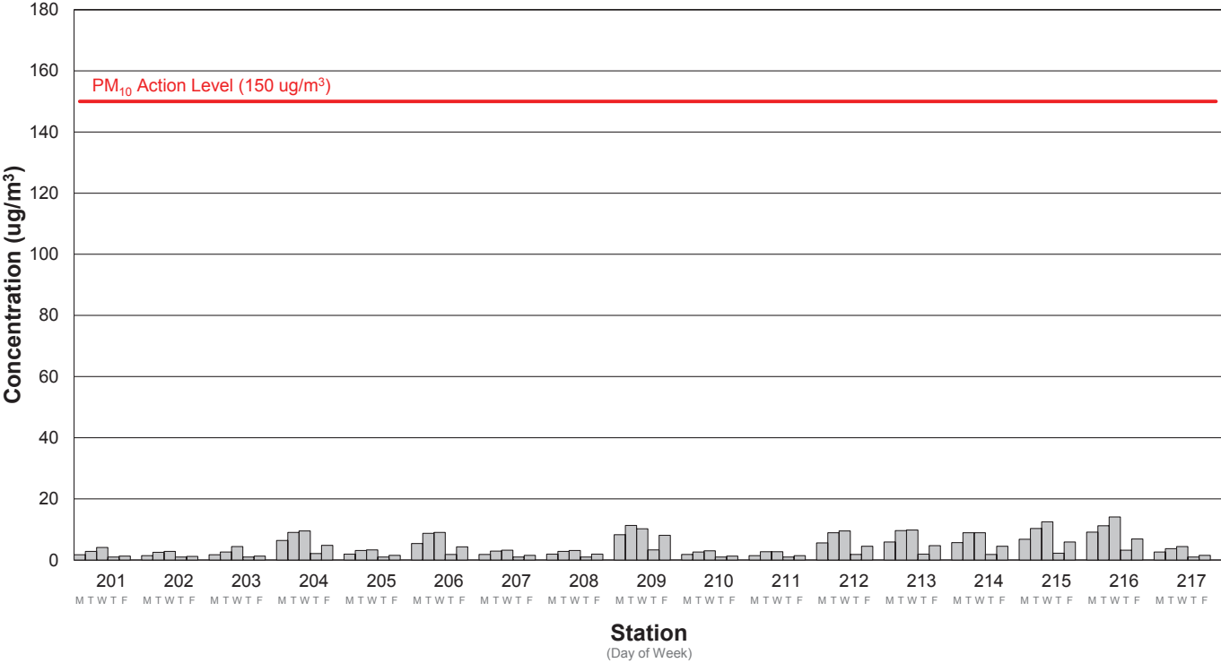
Average PM10 Concentration Week 87: 2/9/2026 - 2/13/2026
